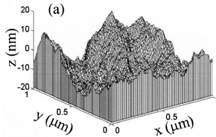
Figure 8 - 3D fractal surface profile [6]
