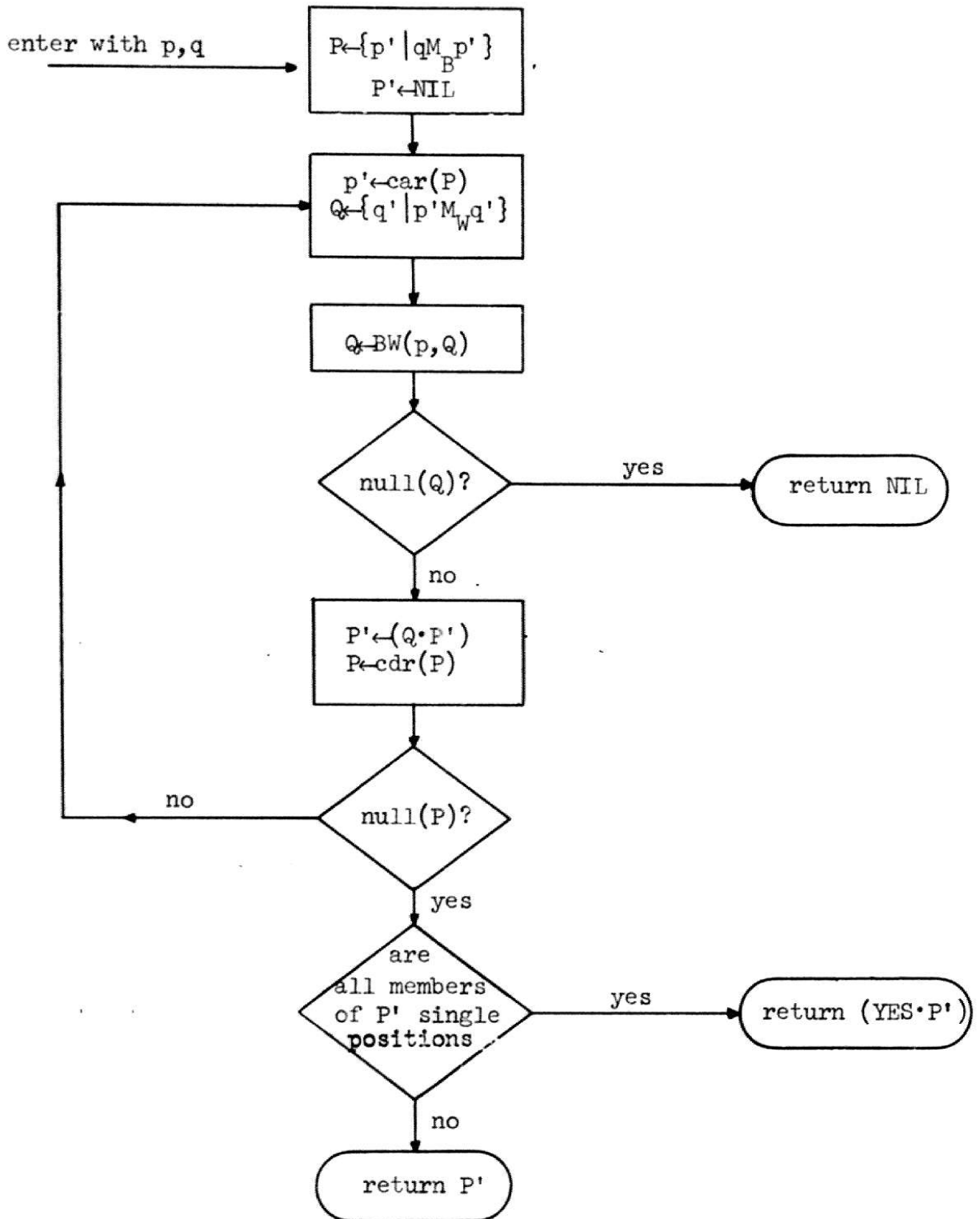
Figure 2.5. Function MB(p,q).q is a single position. Three values are returned.
