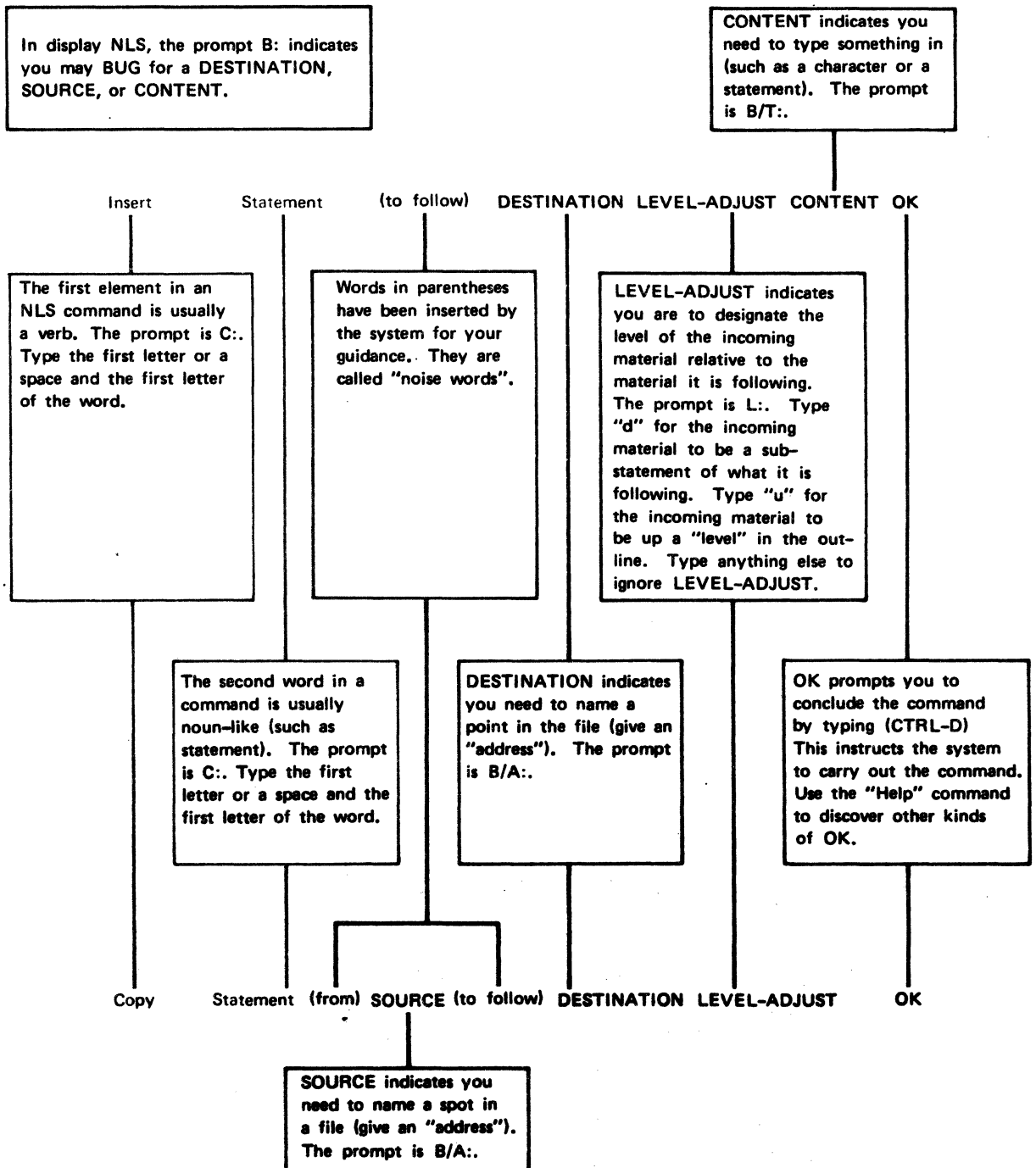
FIGURE 2 COMMAND SYNTAX
