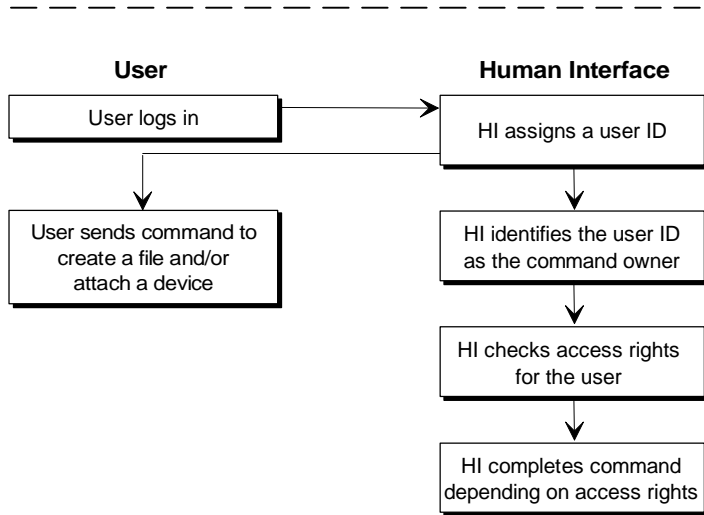
Figure 25-1. Multiuser Support under the HI
