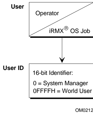
Figure 17-1. User and User ID Relationship
