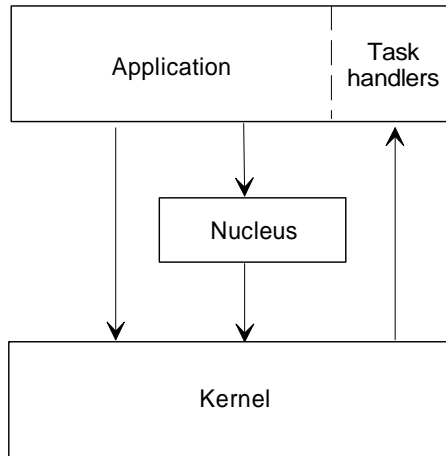
Figure 14-1. Kernel Invoking of Task Handlers
