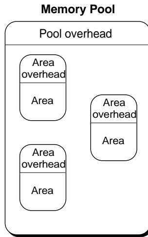
Figure 14-2. Memory Pools and Areas
