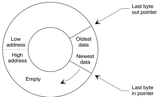
Figure A-1. A Ring Buffer
