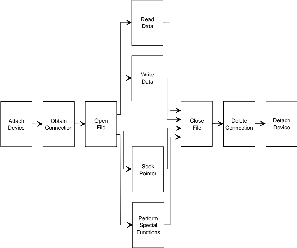
Figure 18-1. Sequence of System Calls for Physical Files
