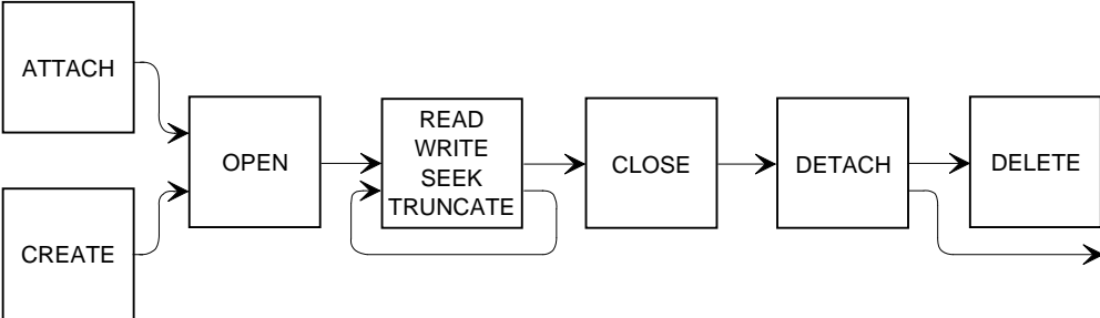
Figure 21-2. Sequence of System Calls for UDI
