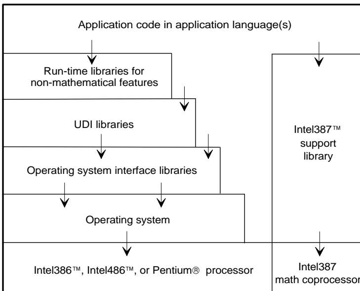
Figure 21-1. The Application Software-Hardware Model
