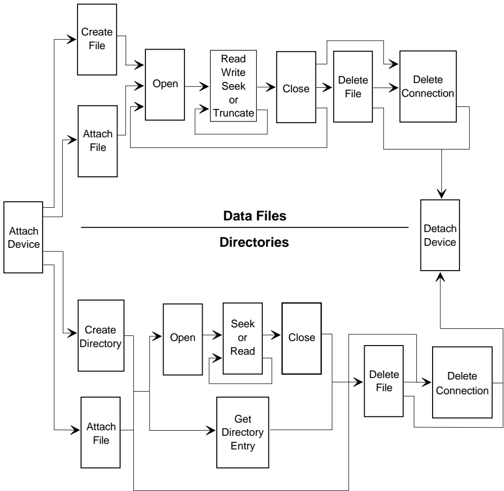
Figure 17-4. Sequence of Frequently Used System Calls for Named Files
