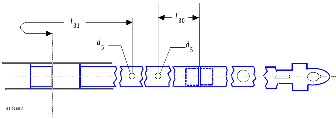
Figure 14 - Leader/tape connection
