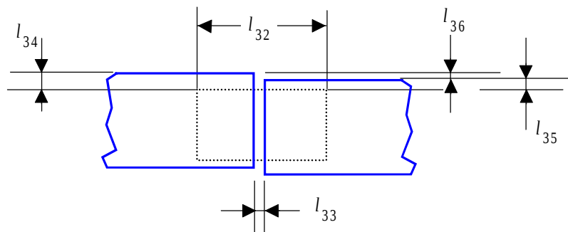
Figure 15 - Position of the splice tape
