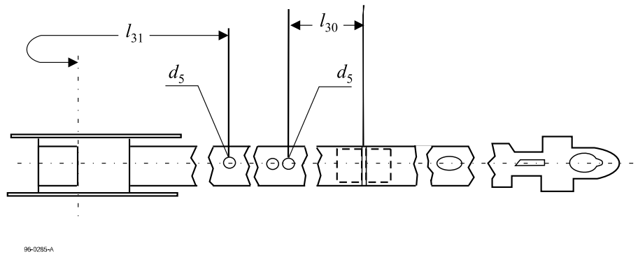
Figure 14 - Leader/tape connection
