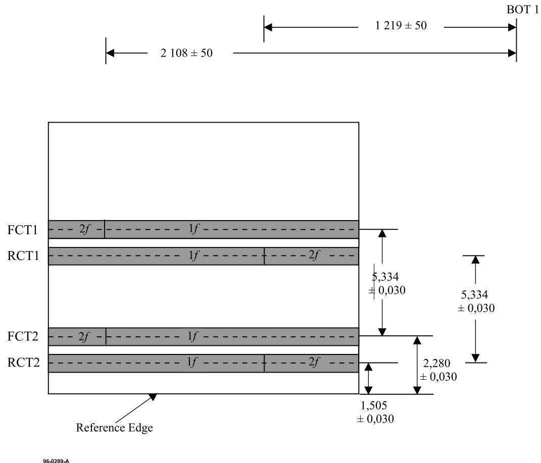
Figure 22 - Calibration Tracks Area
