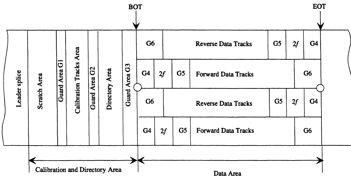
Figure 20 - Tape layout
