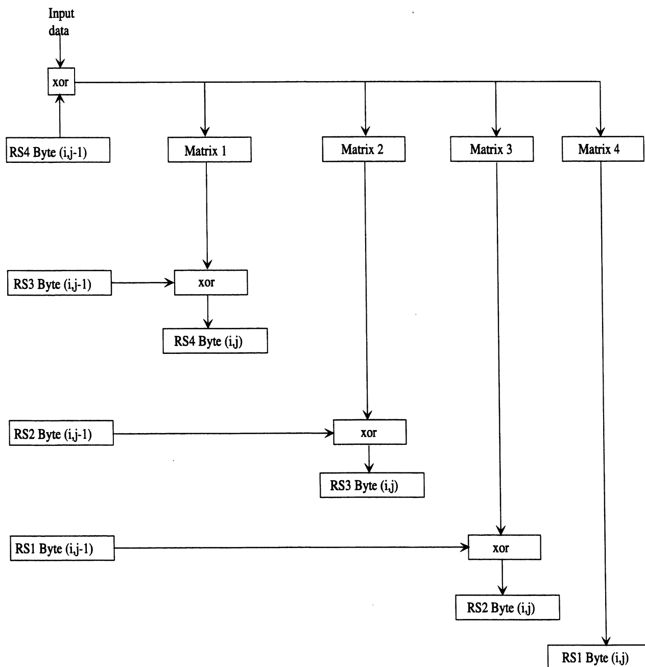
Figure C.1 - ECC Blocks
