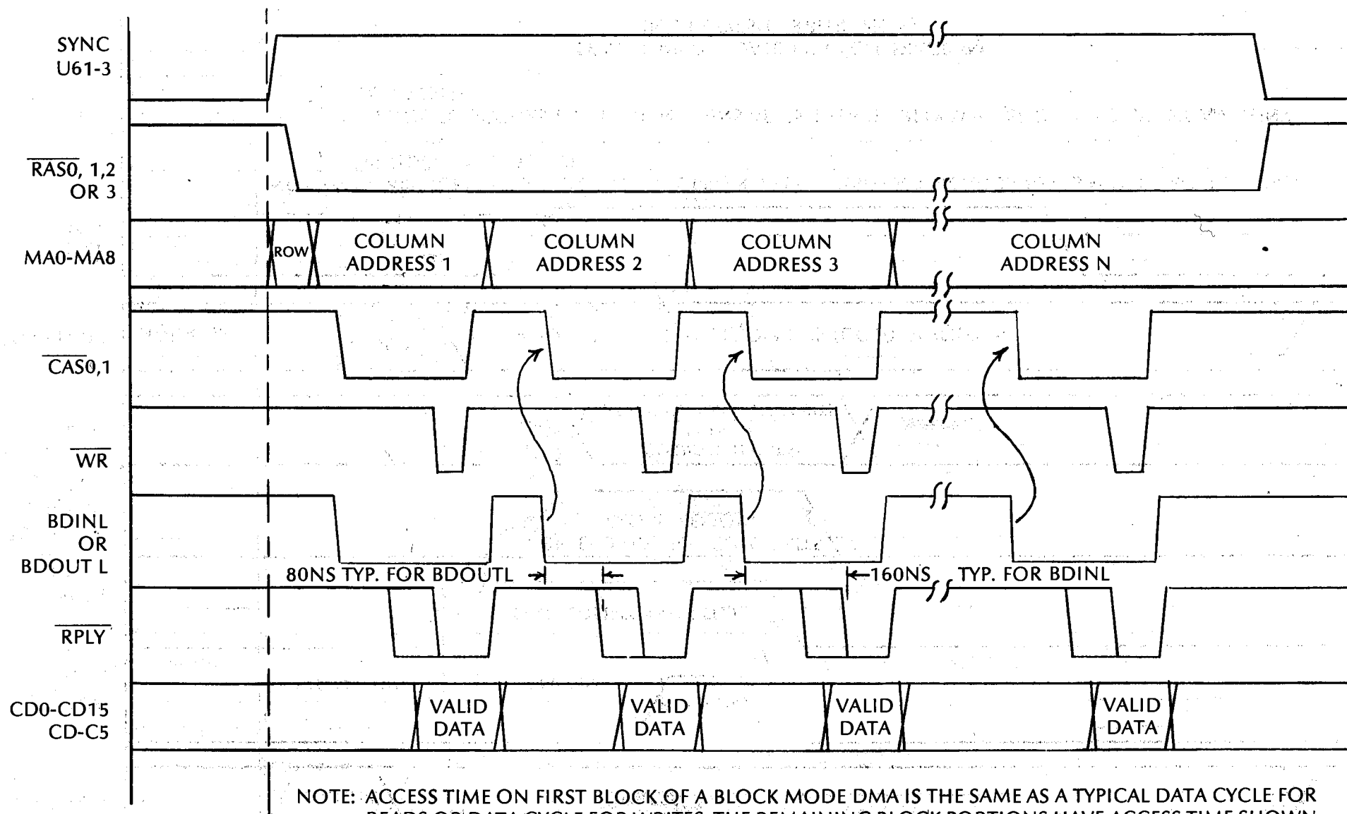
TYPICAL BLOCK MODE DMA CYCLE TIMING (NO REFRESH ARBITRATION)
