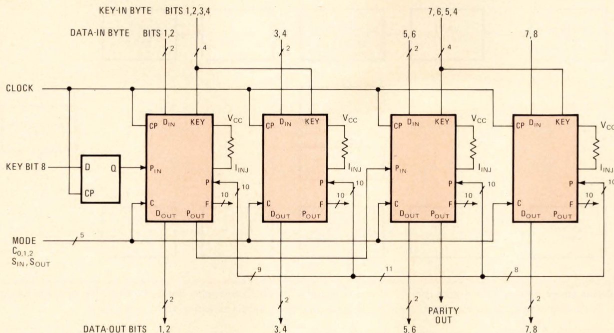
14. Lots of bits. The Fairchild DES implementation is a 4-chip bit-slice approach that takes 4.8 microseconds to encrypt a 64-bit word when driven by a 5-MHz clock. The integrated injection logic on each chip requires 100 milliamperes of injection current.
