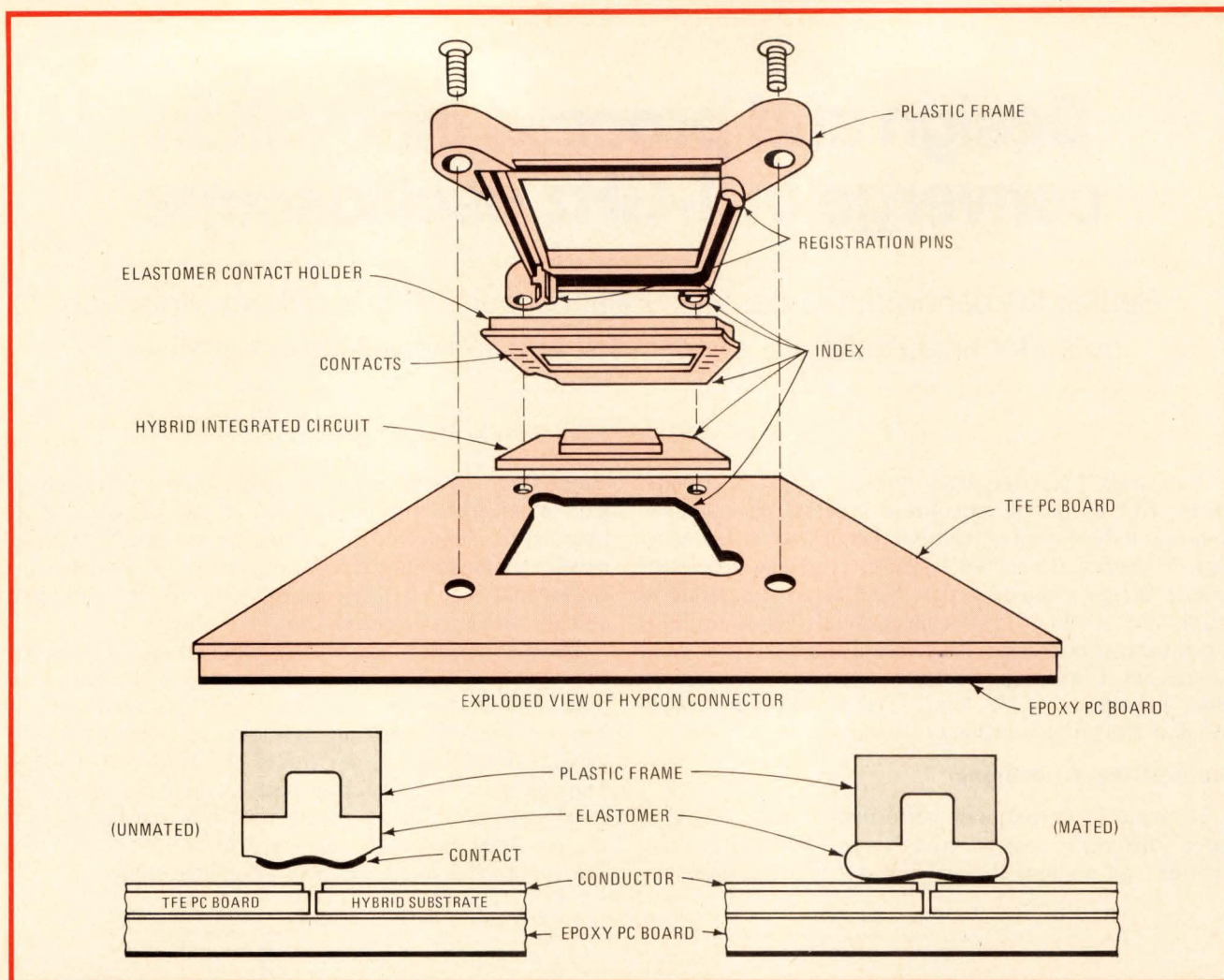
2. Hybrid connection. A Hypcon consists of a glass-impregnated plastic frame that holds a silicone elastomer onto which are bonded gold contacts. These contacts touch both the hybrid package and the printed-circuit conductors without adding appreciable reactance.
