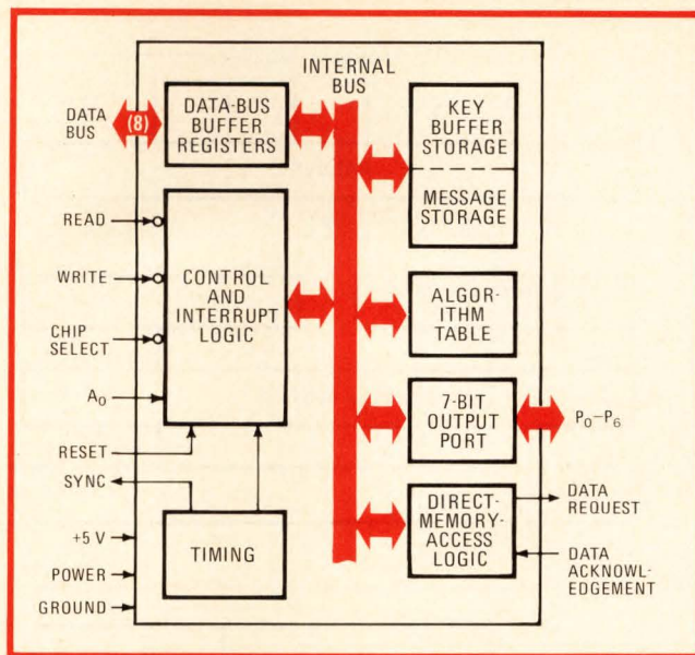
12. Peripheral. Intel's 5-volt device is a microprocessor peripheral with a direct-memory-access interface. Designed for banking applications, this device is byte-oriented, capable of handling up to 80 bytes per second or multiples thereof when paralleled with others.
