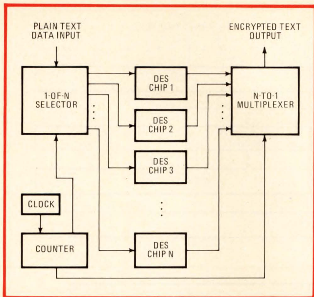
11. High rates. It is possible to multiply the data-handling rates of DES chips by hooking them up as part of a parallel processing circuit. If n chips are used, the effective rate is multiplied by n , but synchronization and timing become critical factors.
