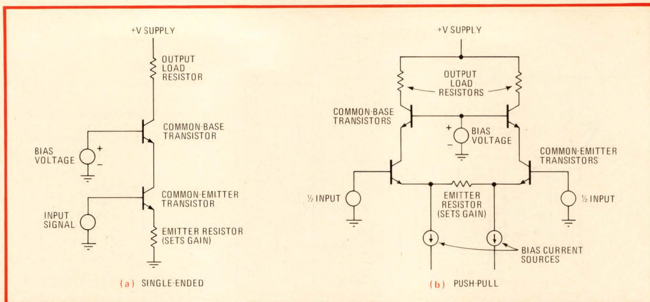
5. Cascode connection. Conventional transistor cascode (a) uses a common-emitter transistor driving a common-base transistor. The push-pull cascode (b) has greater immunity to supply variations when dc coupling is required and always has a zero inductance ground.
