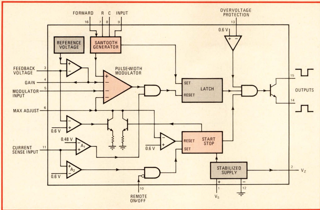
2. Squeezing functions. NE5560 controller provides regulator's switching transistor with frequency-stable output signal having adjustable duty cycle. Maximum duty cycle is programmable. Also included are overload protection, automatic startup after cause for overload is removed, and microprocessor-compatible port for sequential or individual startup of supplies in multiple-output arrangement.
