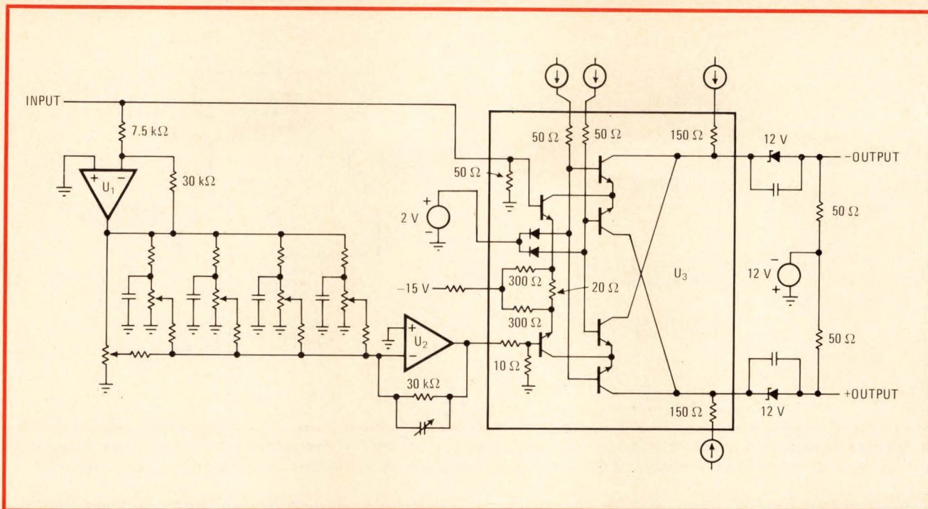
3. Feedbeside. In this technique, low-frequency signals are amplified by operational amplifier U_1 . Different amounts of this signal are selected by five pots and filtered; this voltage is then amplified by U_2 and subtracted from the wideband input by U_3 .
