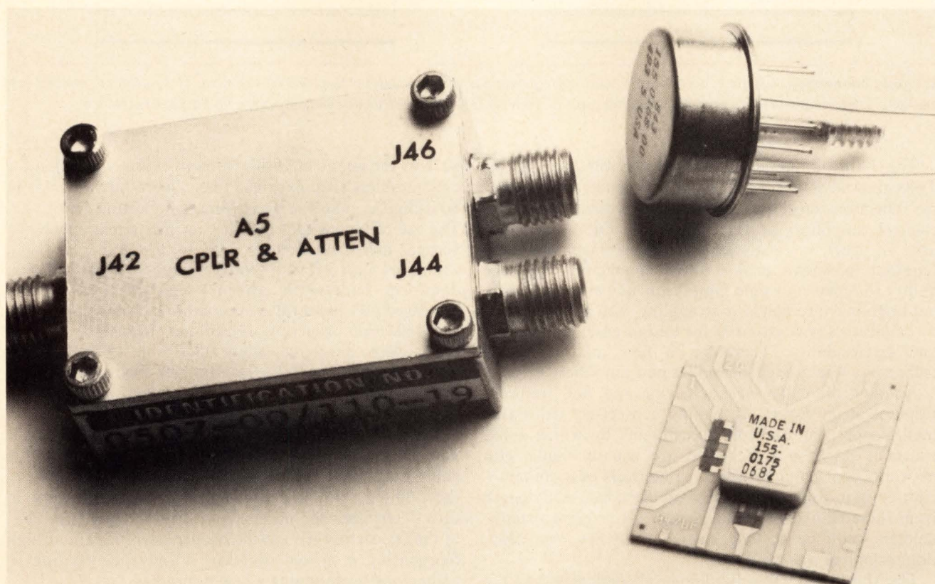
1. Hybrid packages. At the left is an aluminum box typical of those used in spectrum analyzers and other microwave systems. Upper right is a package typical of those used in the 7904 500-MHz oscilloscope. Below is a new hybrid package basic to the 7104 1-GHz scope.
