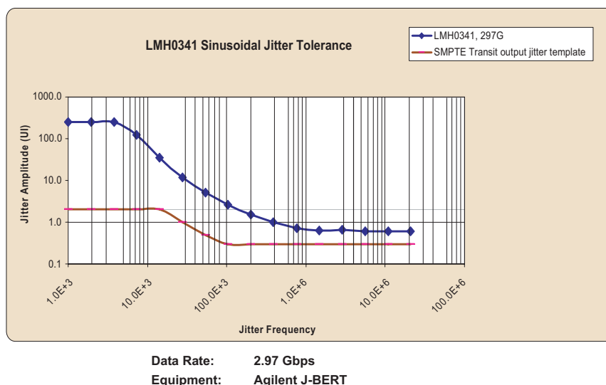
Figure 2 – LMH0341 minimum input jitter tolerance: 0.6 UI
