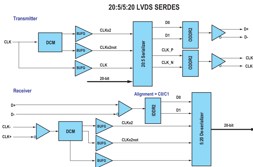
Figure 4 – Basic soft SERDES construct in Spartan-3E FPGAs
