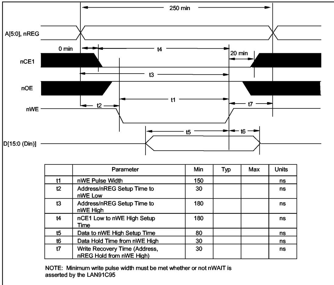
FIGURE 19 - PCMCIA MEMORY WRITE TIMING
