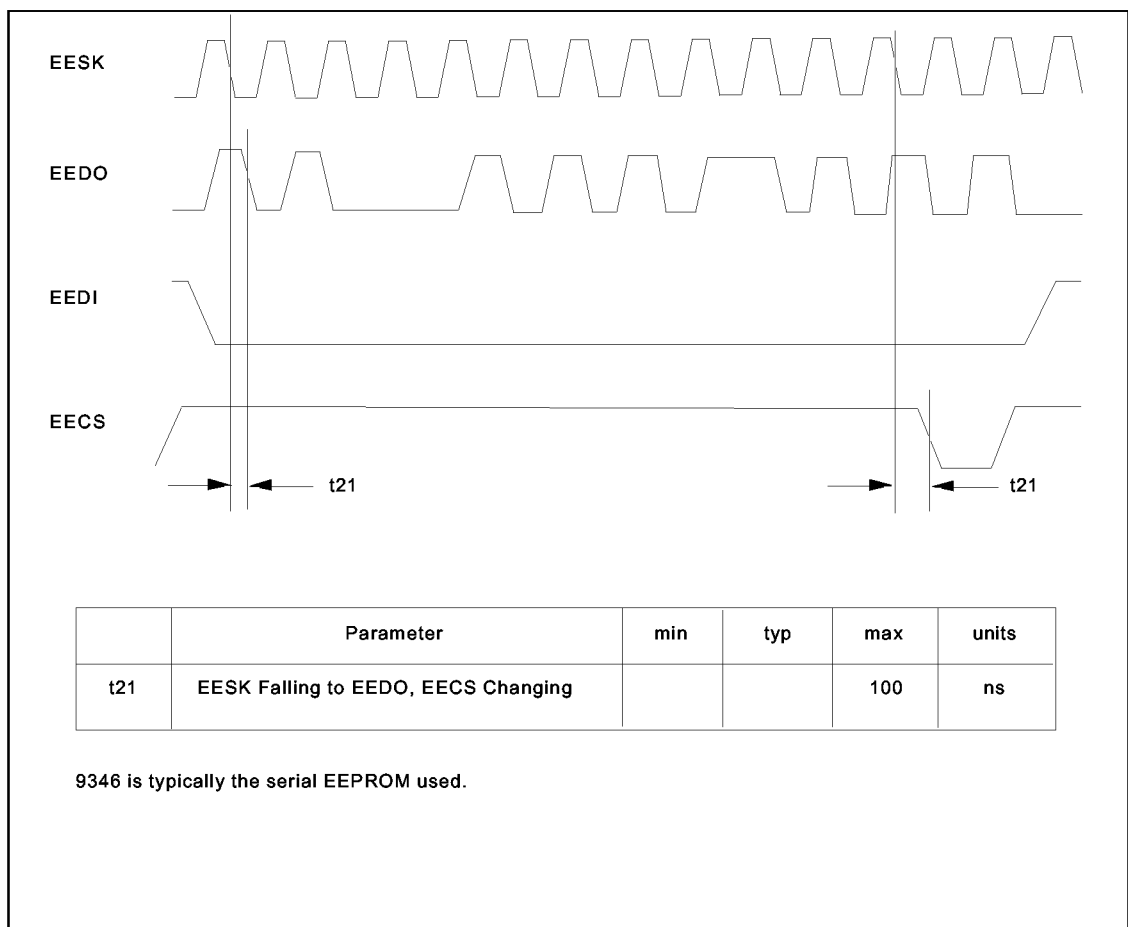
FIGURE 37 - EEPROM WRITE
