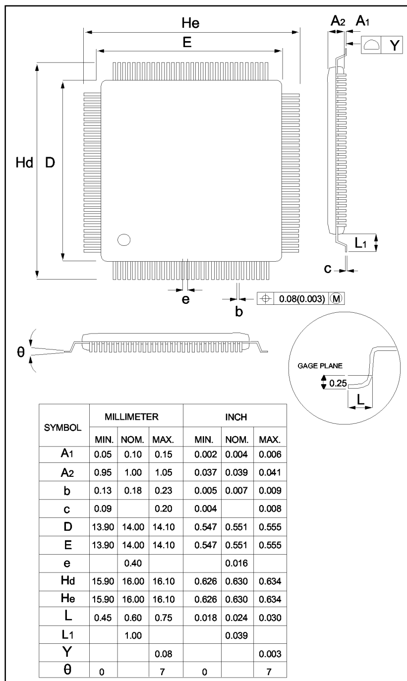
FIGURE 47 - VTQFP PACKAGE OUTLINE
