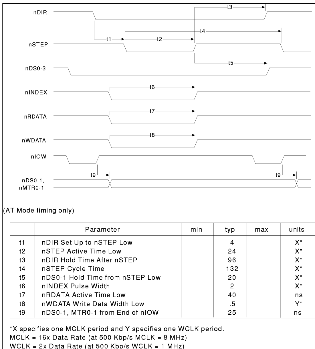
FIGURE 8 - DISK DRIVE TIMING
