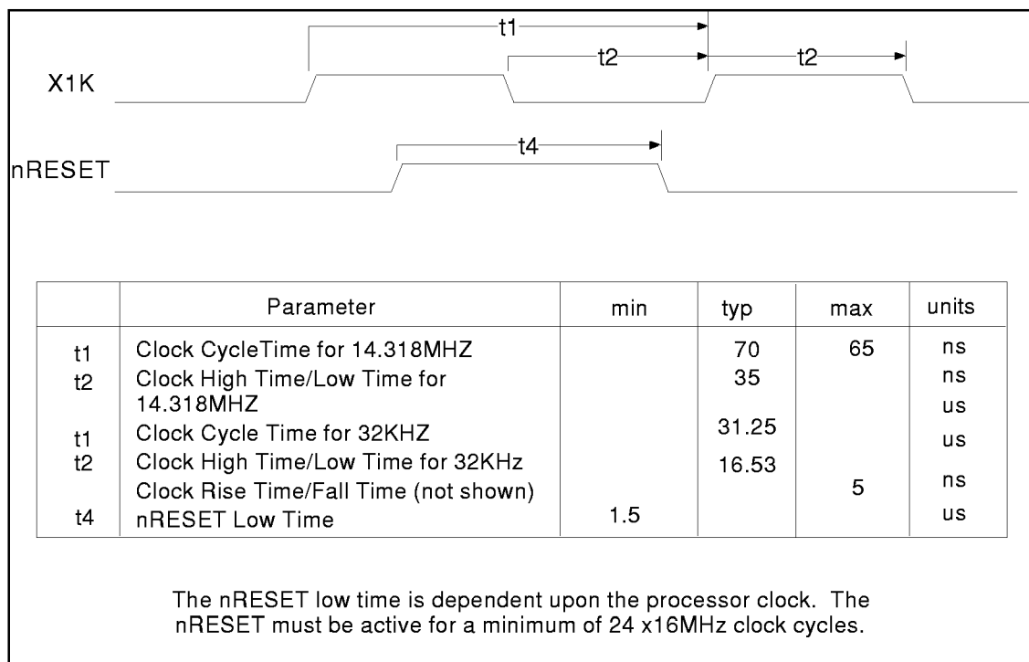
FIGURE 7 - CLOCK TIMING
