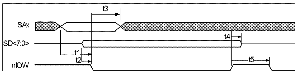
FIGURE 2 - IOW TIMING FOR PORT 92
