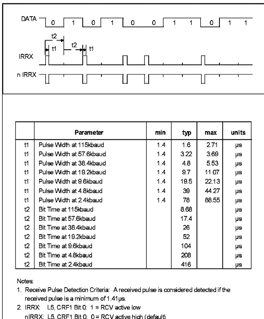
FIGURE 19 - IrDA RECEIVE TIMING
