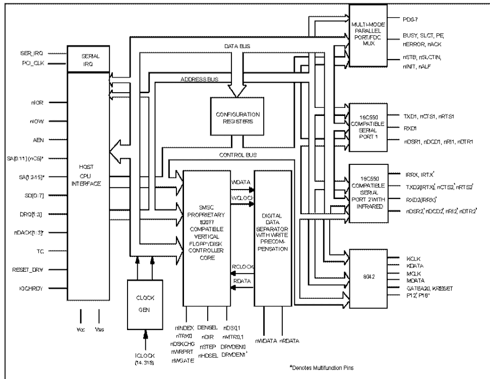
FIGURE 1 - FDC37M60x BLOCK DIAGRAM
