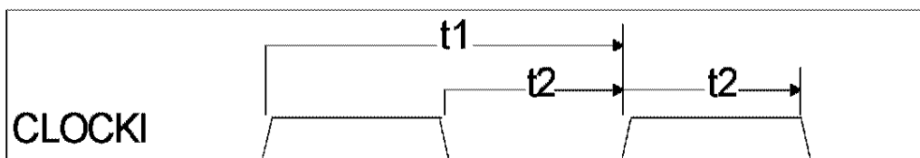
FIGURE 7A - INPUT CLOCK TIMING
