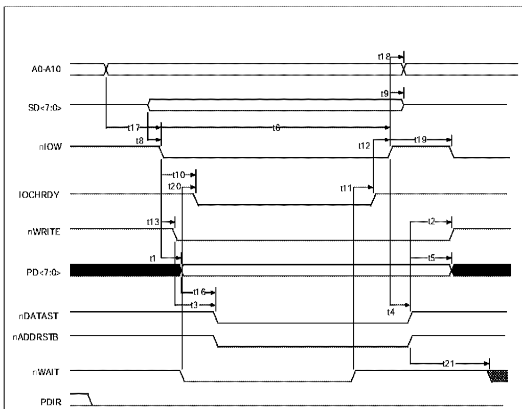
FIGURE 14A - EPP 1.7 DATA OR ADDRESS WRITE CYCLE
