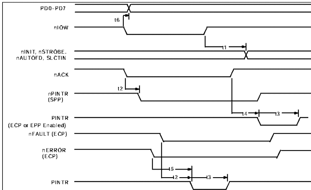
FIGURE 11 - PARALLEL PORT TIMING
