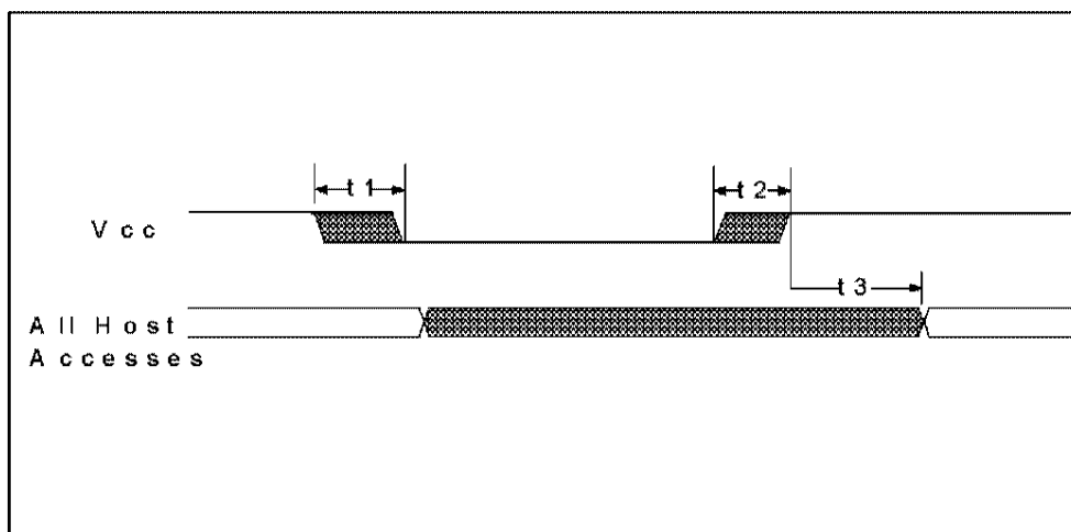
FIGURE 3 - POWER-UP TIMING
