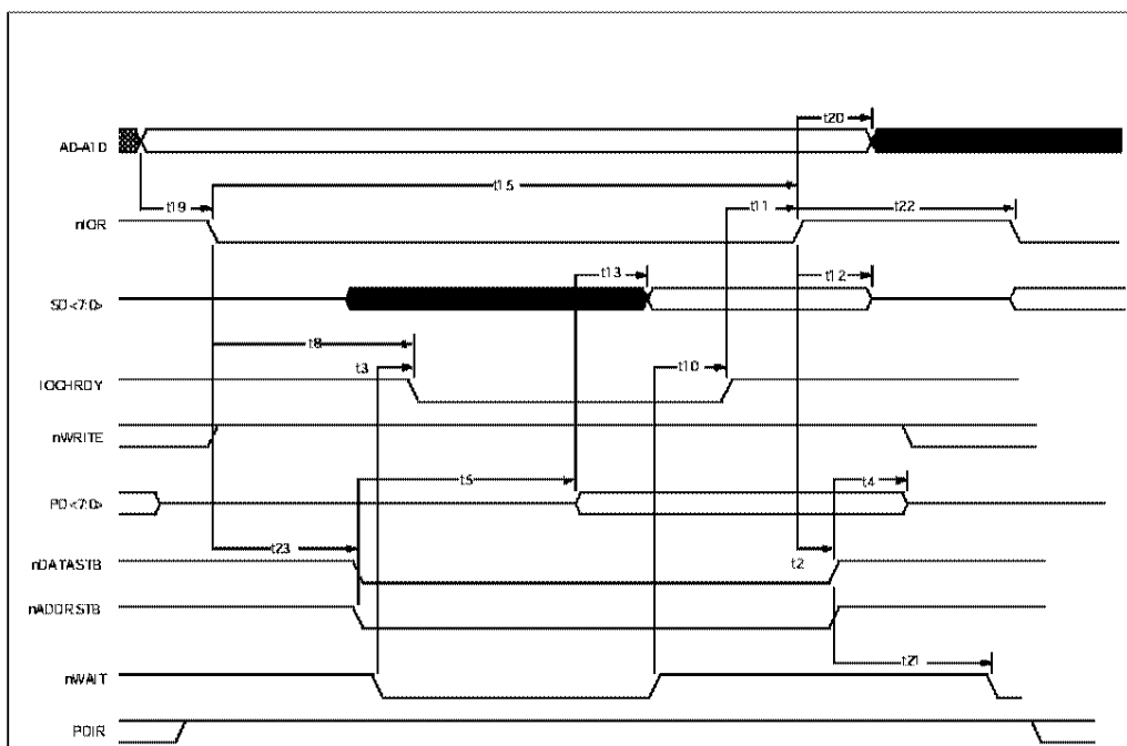
FIGURE 15A - EPP 1.7 DATA OR ADDRESS READ CYCLE
