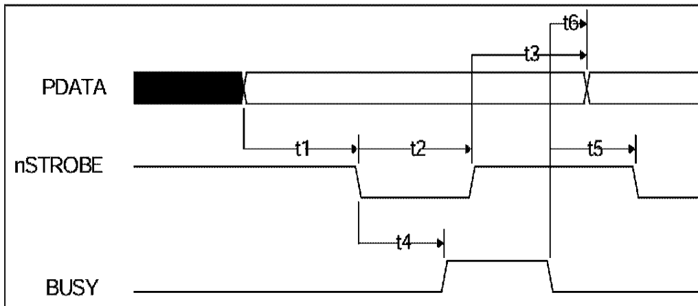
FIGURE 16 - PARALLEL PORT FIFO TIMING
