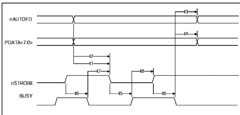
FIGURE 17 - ECP PARALLEL PORT FORWARD TIMING
