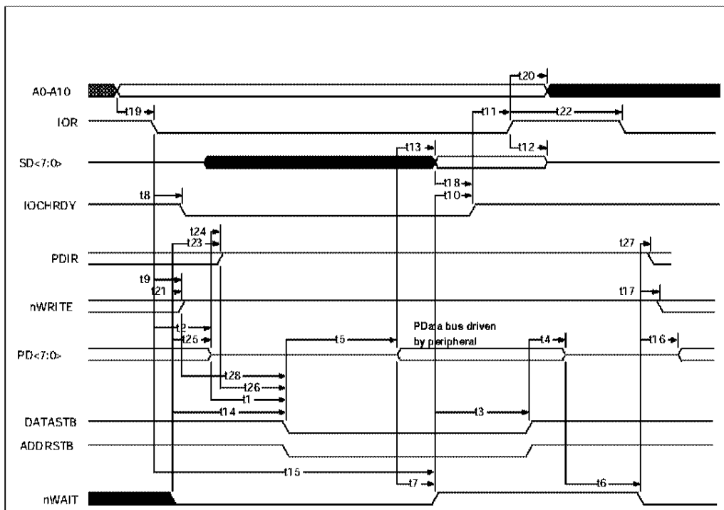
FIGURE 13A - EPP 1.9 DATA OR ADDRESS READ CYCLE
