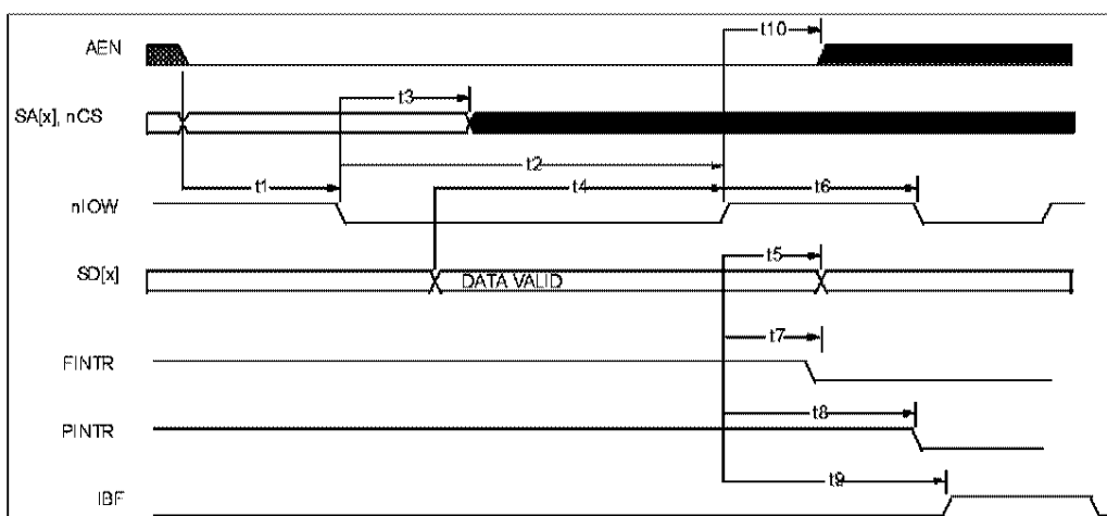
FIGURE 4 - ISA WRITE
