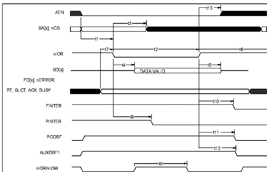
FIGURE 5 - ISA READ
