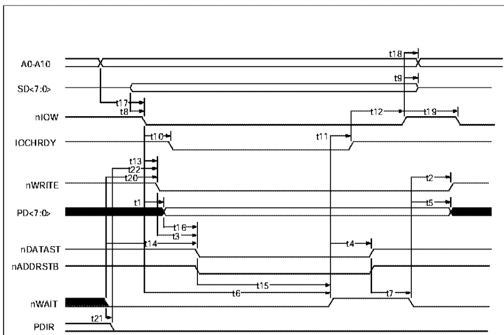
FIGURE 12A - EPP 1.9 DATA OR ADDRESS WRITE CYCLE
