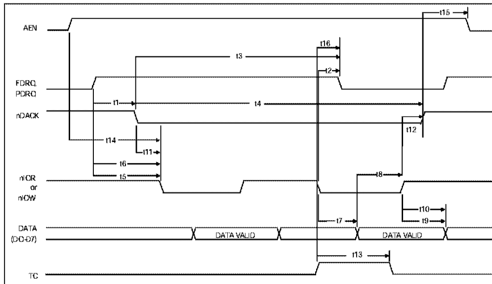
FIGURE 8B - DMA TIMING (BURST TRANSFER MODE)
