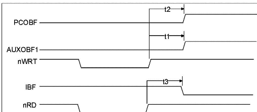
FIGURE 6 - INTERNAL 8042 CPU TIMING
