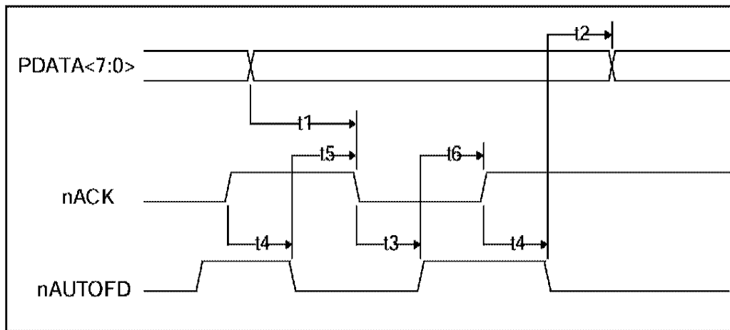
FIGURE 18 - ECP PARALLEL PORT REVERSE TIMING
