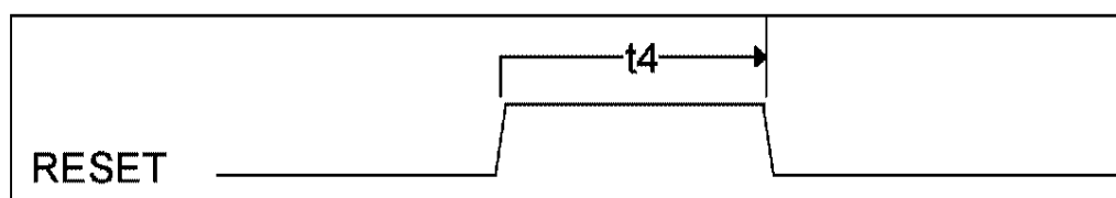
FIGURE 21B - RESET TIMING
