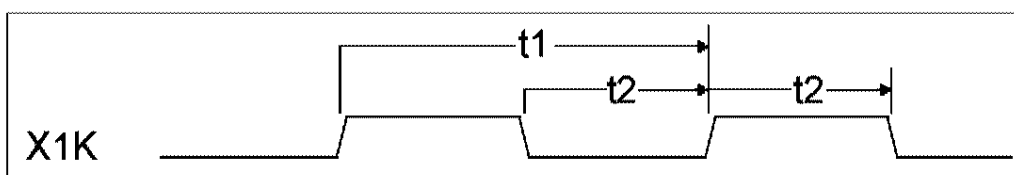
FIGURE 21A - INPUT CLOCK TIMING
