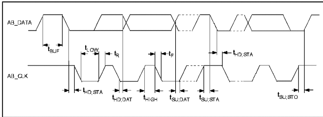
FIGURE 37 - ACCESS.BUS TIMING
