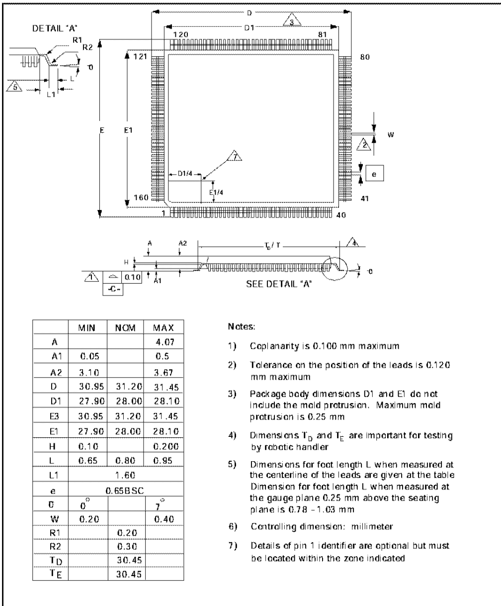
FIGURE 42 - 160 PIN QFP PACKAGE OUTLINES
