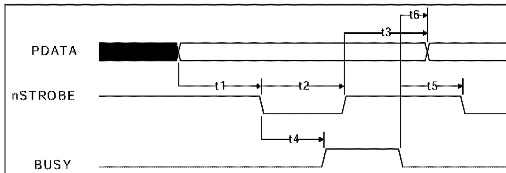
FIGURE 34 - PARALLEL PORT FIFO TIMING
