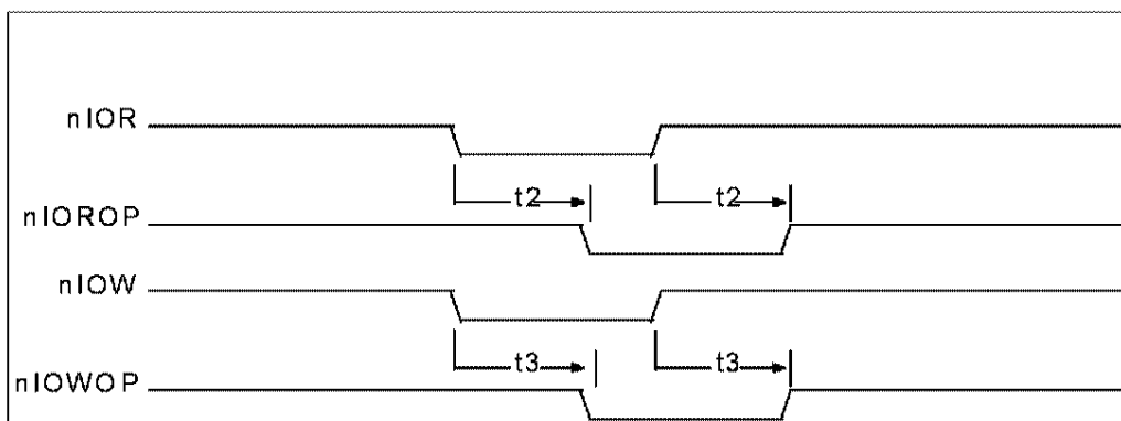
FIGURE 23 - nIOROP, nIOWOP TIMING
