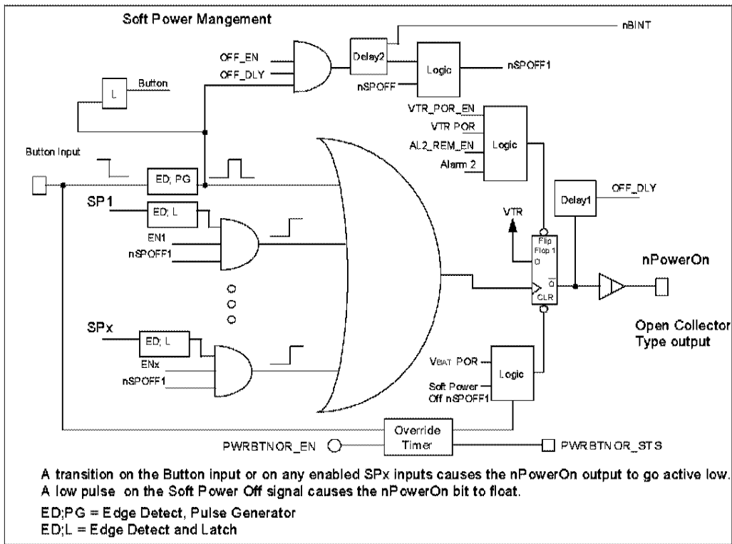
FIGURE 11 - SOFT POWER MANAGEMENT FUNCTIONAL DIAGRAM
