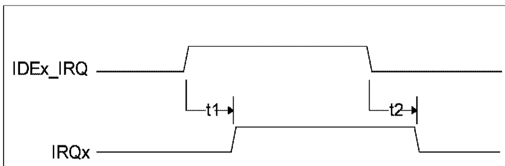
FIGURE 22 - IRQ TIMING
