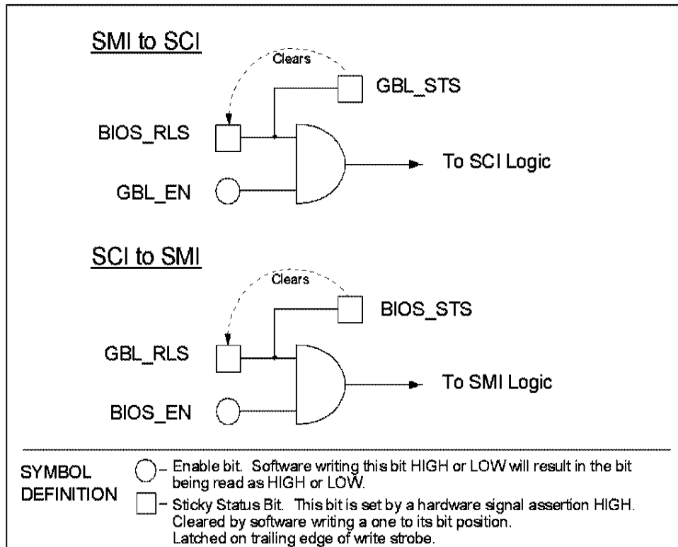
FIGURE 13 - PROCESS OF GENERATING AN INTERRUPT FROM SMI TO SCI AND SCI TO SMI
