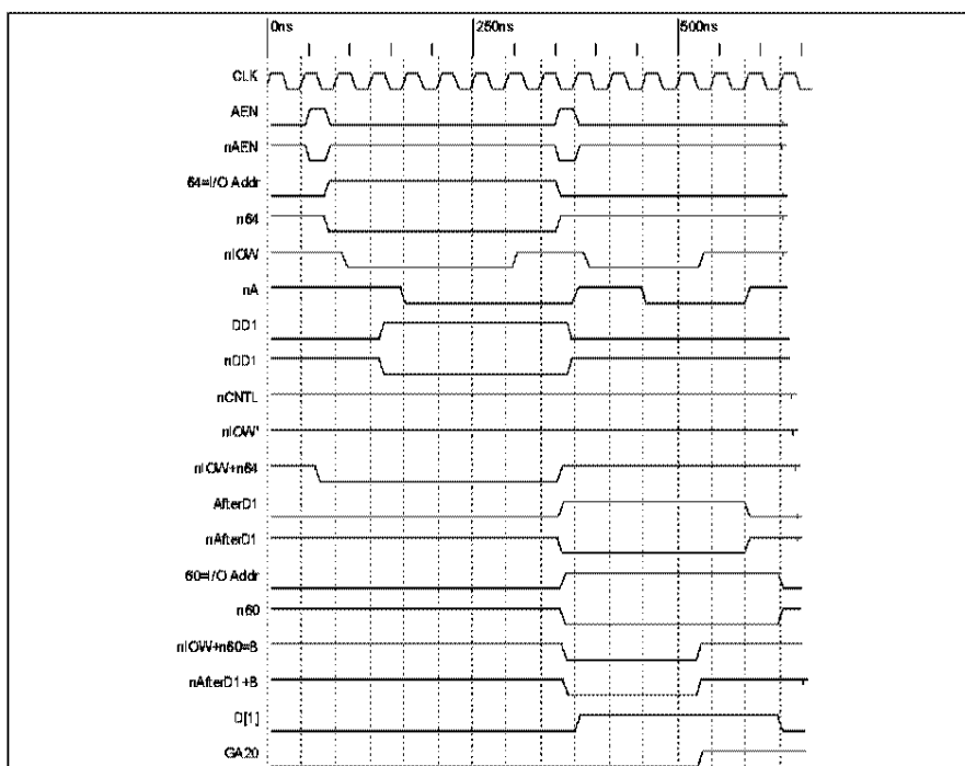
FIGURE 9 - GATE A20 TURN-ON SEQUENCE TIMING
