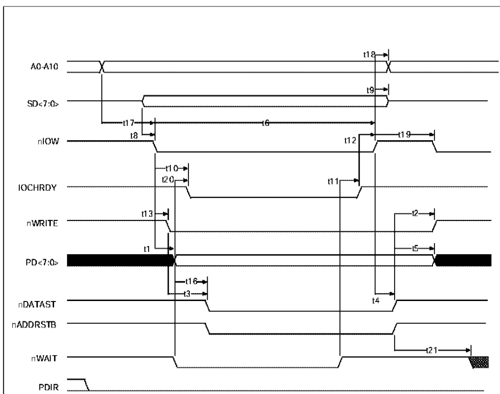
FIGURE 32A - EPP 1.7 DATA OR ADDRESS WRITE CYCLE
