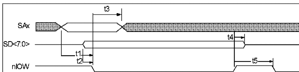
FIGURE 16 - IOW TIMING FOR PORT 92
