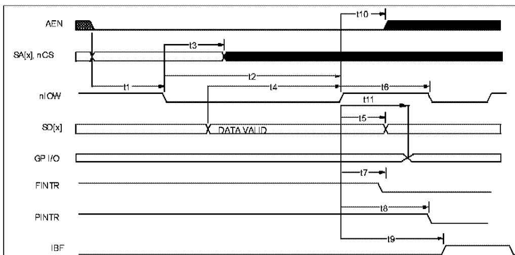
FIGURE 18 - ISA WRITE
