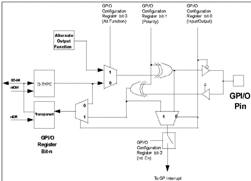
FIGURE 5 - GPIO HAVING AN OUTPUT-TYPE ALTERNATE FUNCTION [GP12 - GP17, GP20, GP22 - GP25]
