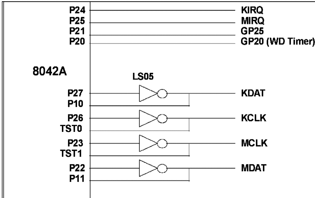
FIGURE 6 - KEYBOARD AND MOUSE INTERFACE
