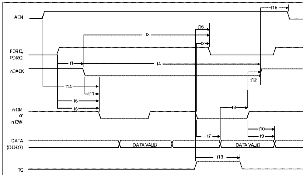
FIGURE 25B - DMA TIMING (BURST TRANSFER MODE)
