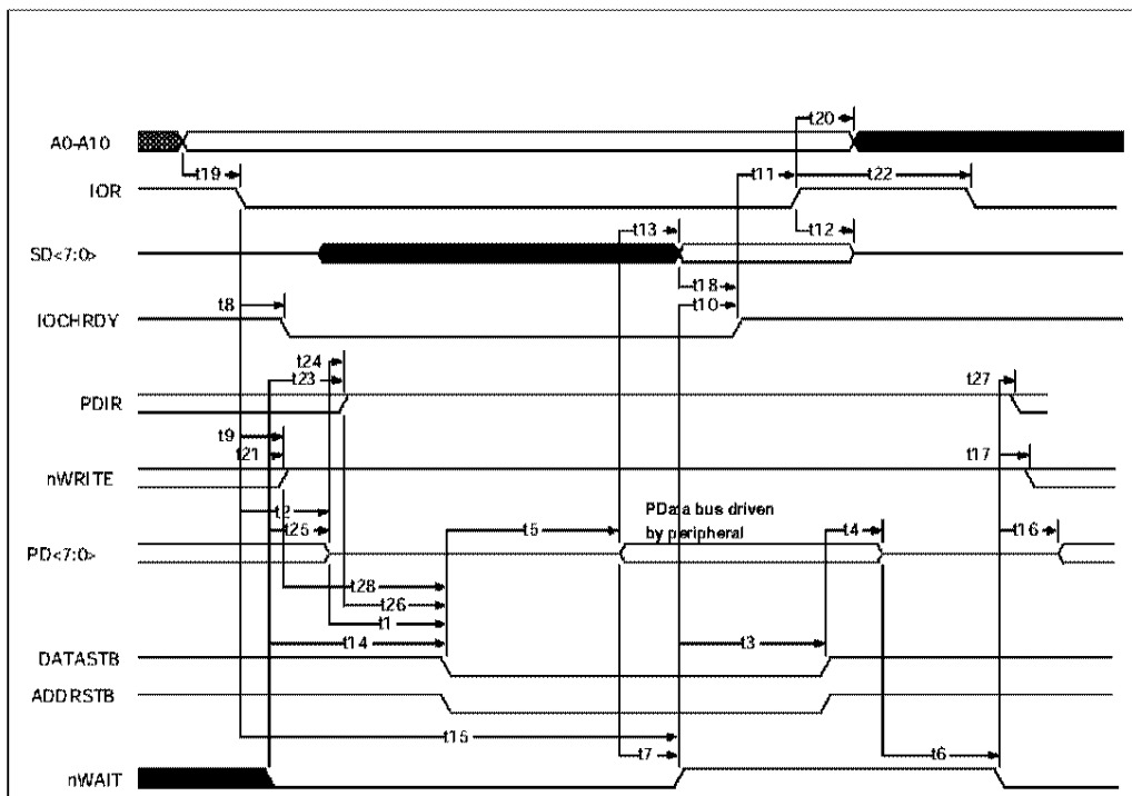
FIGURE 31A - EPP 1.9 DATA OR ADDRESS READ CYCLE
