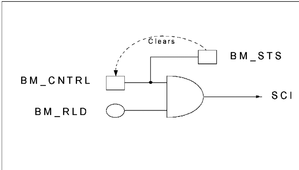
FIGURE 14 - BUS MASTER SCI EVENT LOGIC
