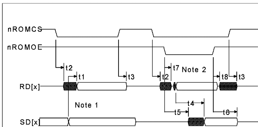
FIGURE 24 - ROM INTERFACE TIMING
