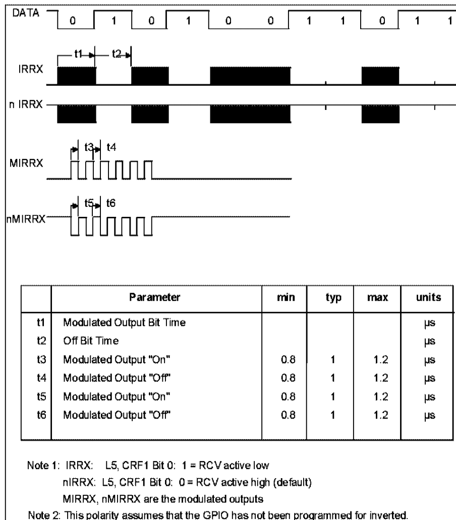
FIGURE 40 - AMPLITUDE SHIFT KEYED IR RECEIVE TIMING
