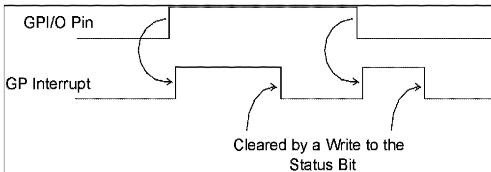
FIGURE 6 - EITHER EDGE TRIGGERED INTERRUPT TIMING EXAMPLE
