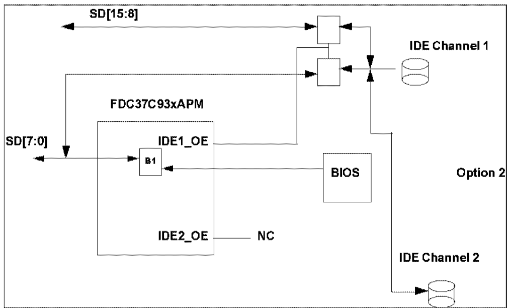
FIGURE 3 - IDE OUTPUT ENABLE OPTION 2
