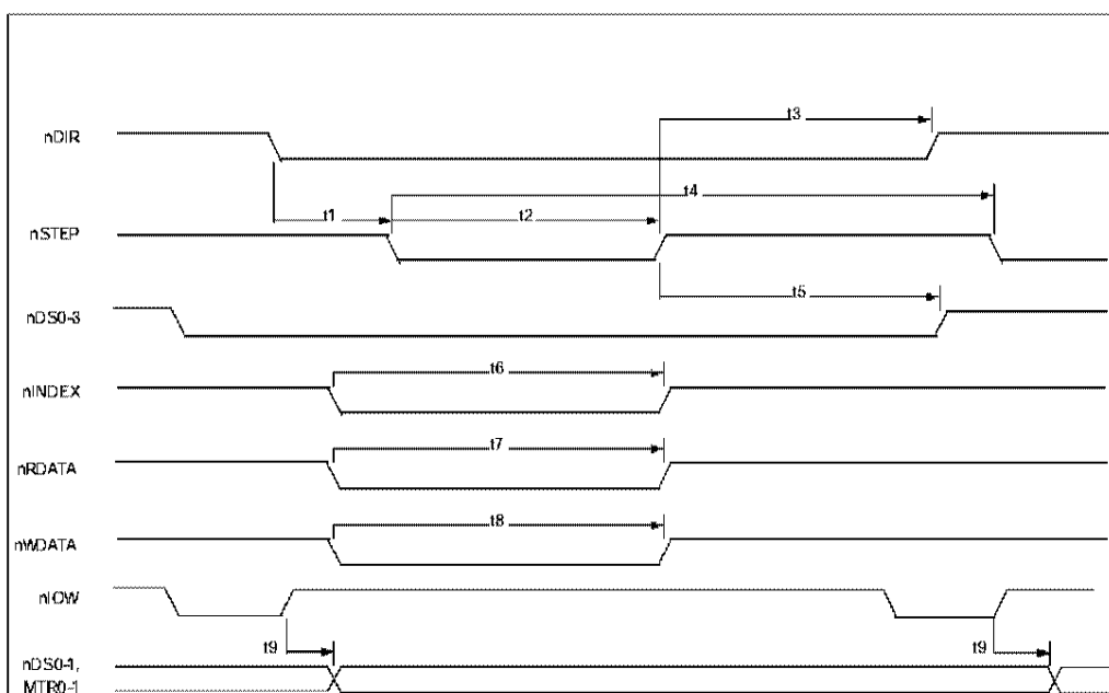
FIGURE 26 - DISK DRIVE TIMING (AT MODE ONLY)
