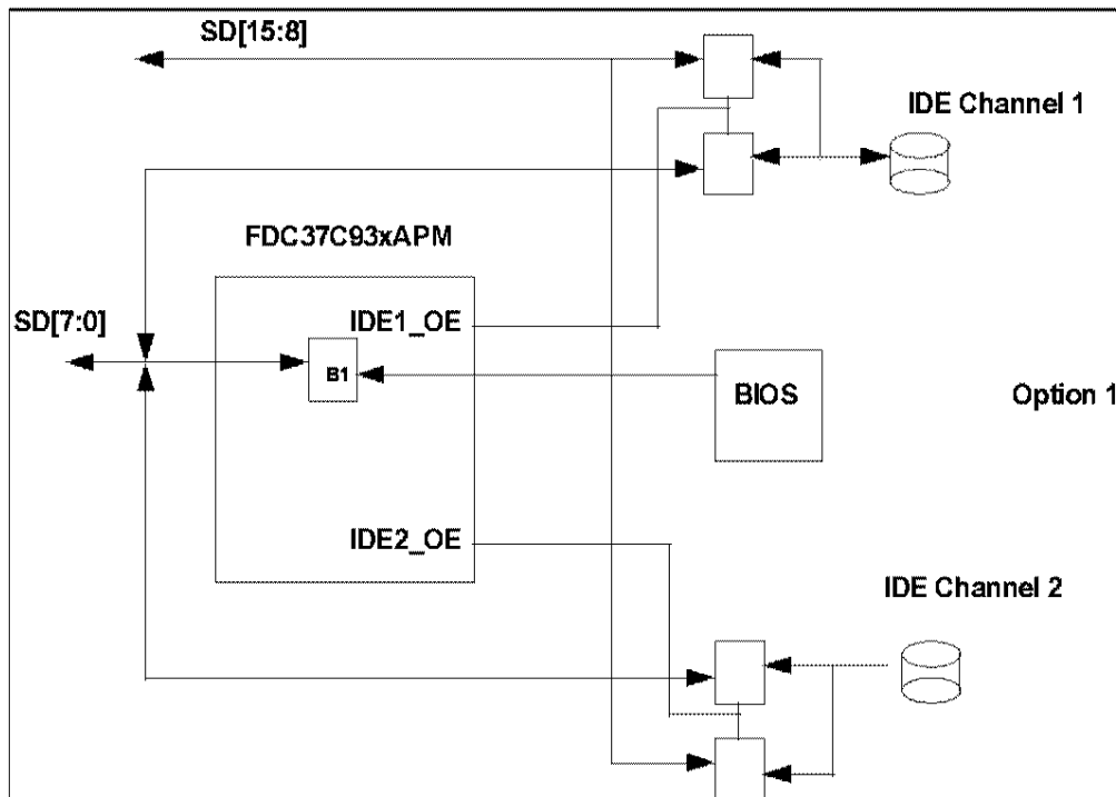
FIGURE 2 - IDE OUTPUT ENABLE OPTION 1I
