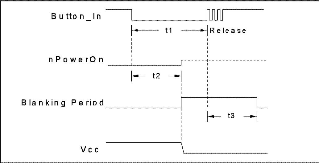
FIGURE 15B - BUTTON OVERRIDE TIMING
