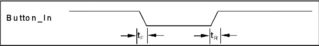
FIGURE 15A - BUTTON INPUT TIMING
