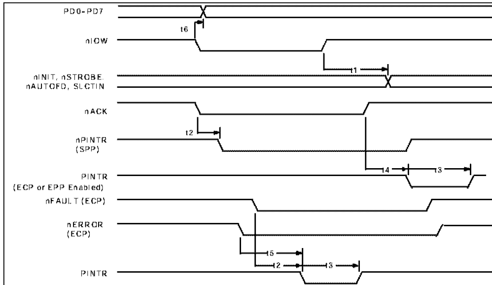
FIGURE 29 - PARALLEL PORT TIMING
