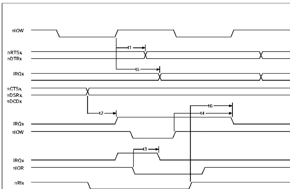
FIGURE 27 - SERIAL PORT TIMING
