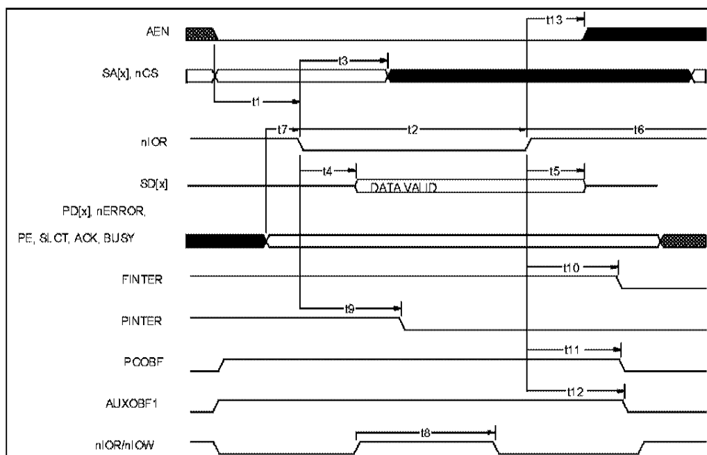
FIGURE 19 - ISA READ
