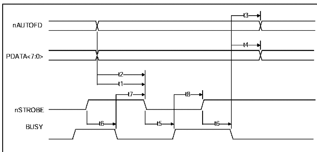
FIGURE 35 - ECP PARALLEL PORT FORWARD TIMING
