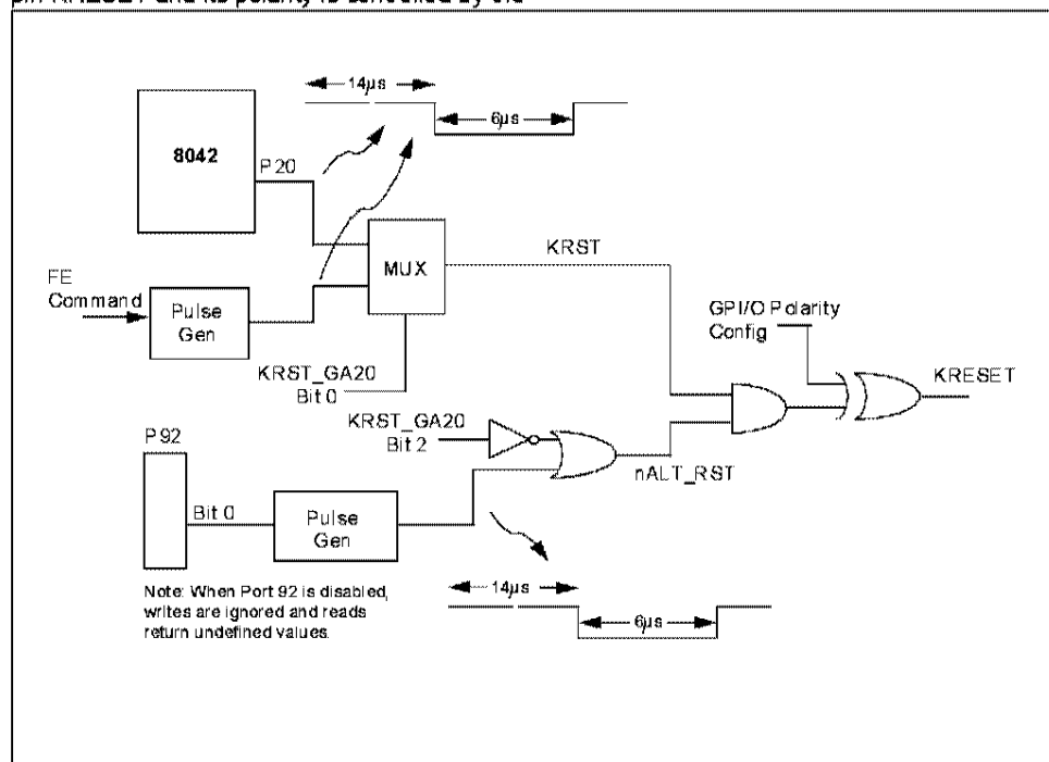
FIGURE 7 - KRESET GENERATION
