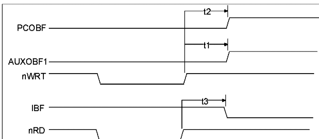
FIGURE 20 - INTERNAL 8042 CPU TIMING
