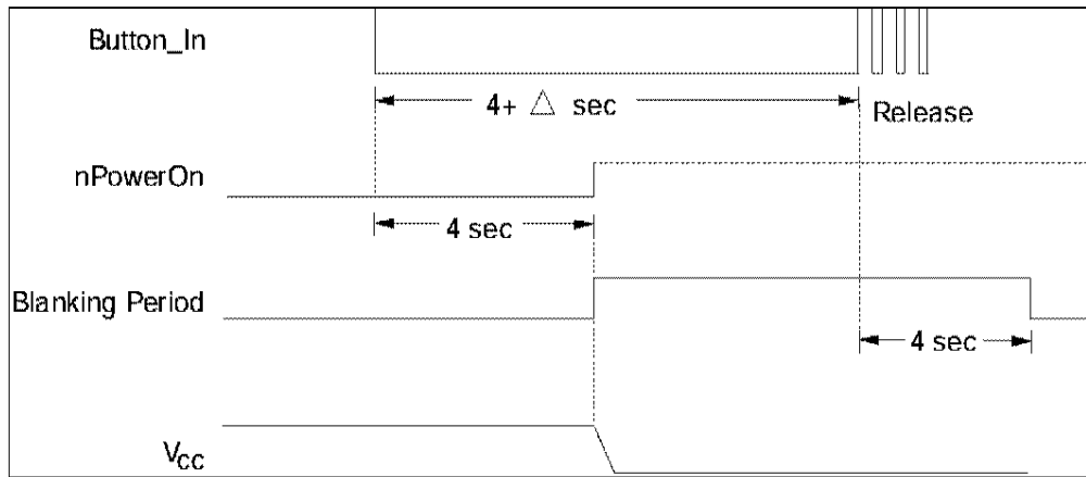
FIGURE 12 - BLANKING PERIOD
