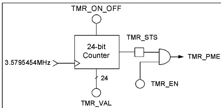
FIGURE 15 - POWER MANAGEMENT TIMER
