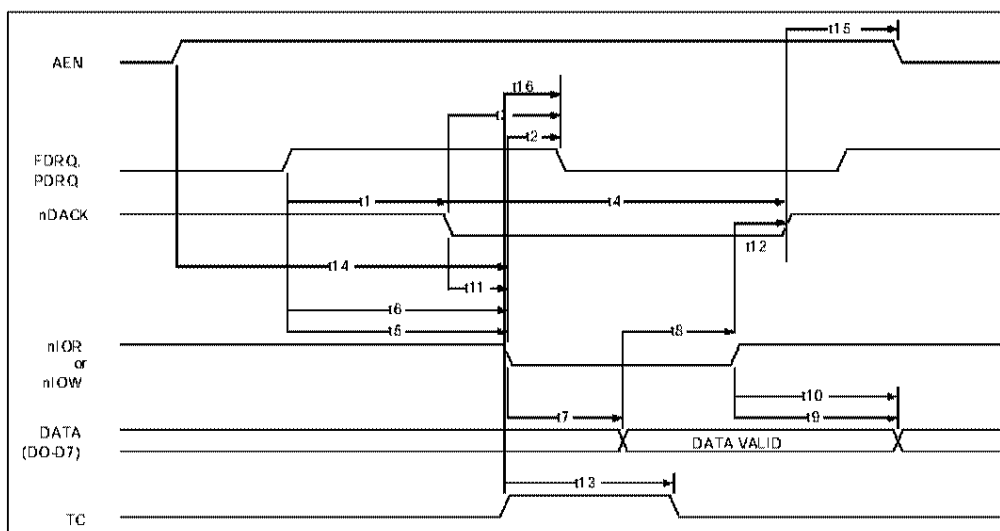
FIGURE 25A - DMA TIMING (SINGLE TRANSFER MODE)
