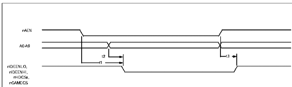
FIGURE 28 - IDE INTERFACE TIMING
