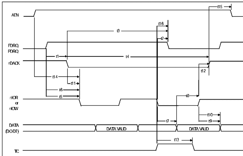
FIGURE 6B - DMA TIMING (BURST TRANSFER MODE)
