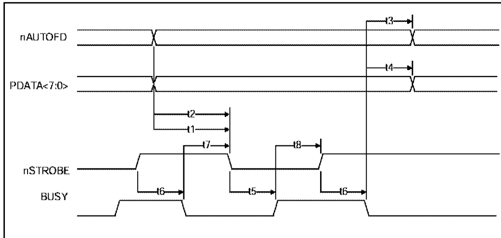
FIGURE 15 - ECP PARALLEL PORT FORWARD TIMING
