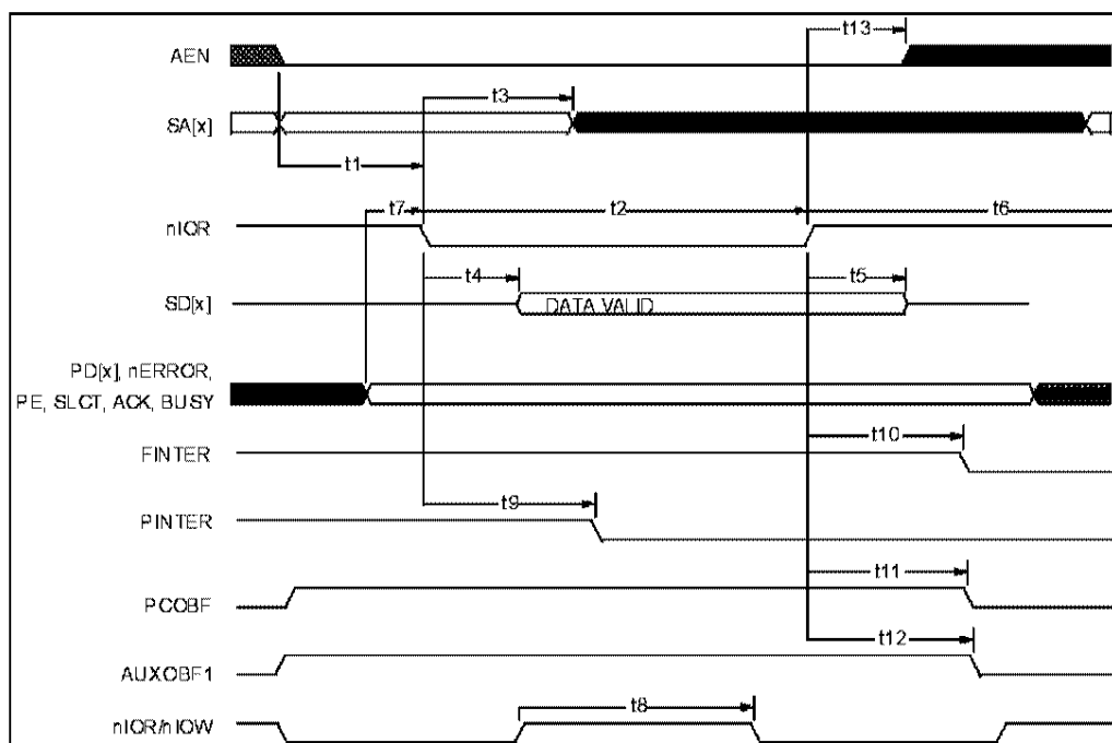
FIGURE 3 - ISA READ
