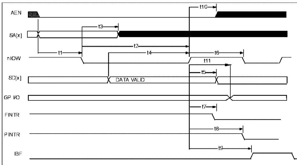
FIGURE 2 - ISA WRITE
