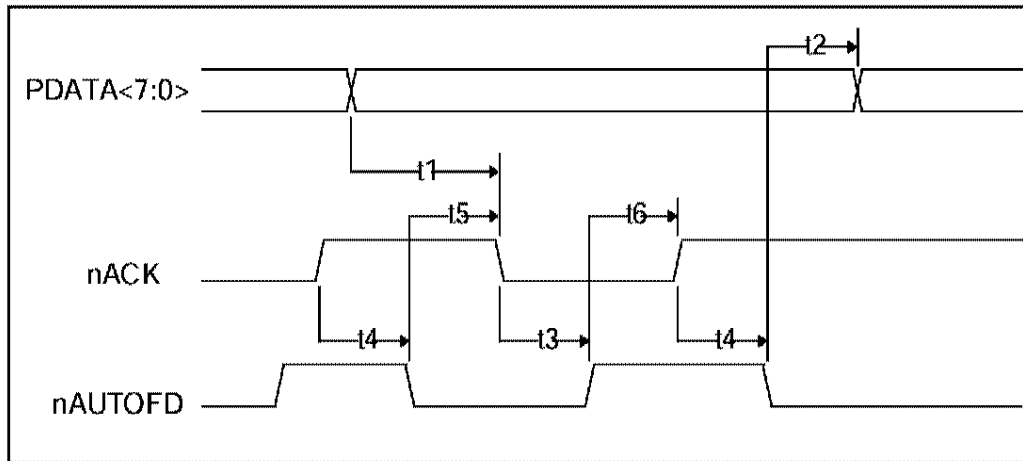
FIGURE 16 - ECP PARALLEL PORT REVERSE TIMING
