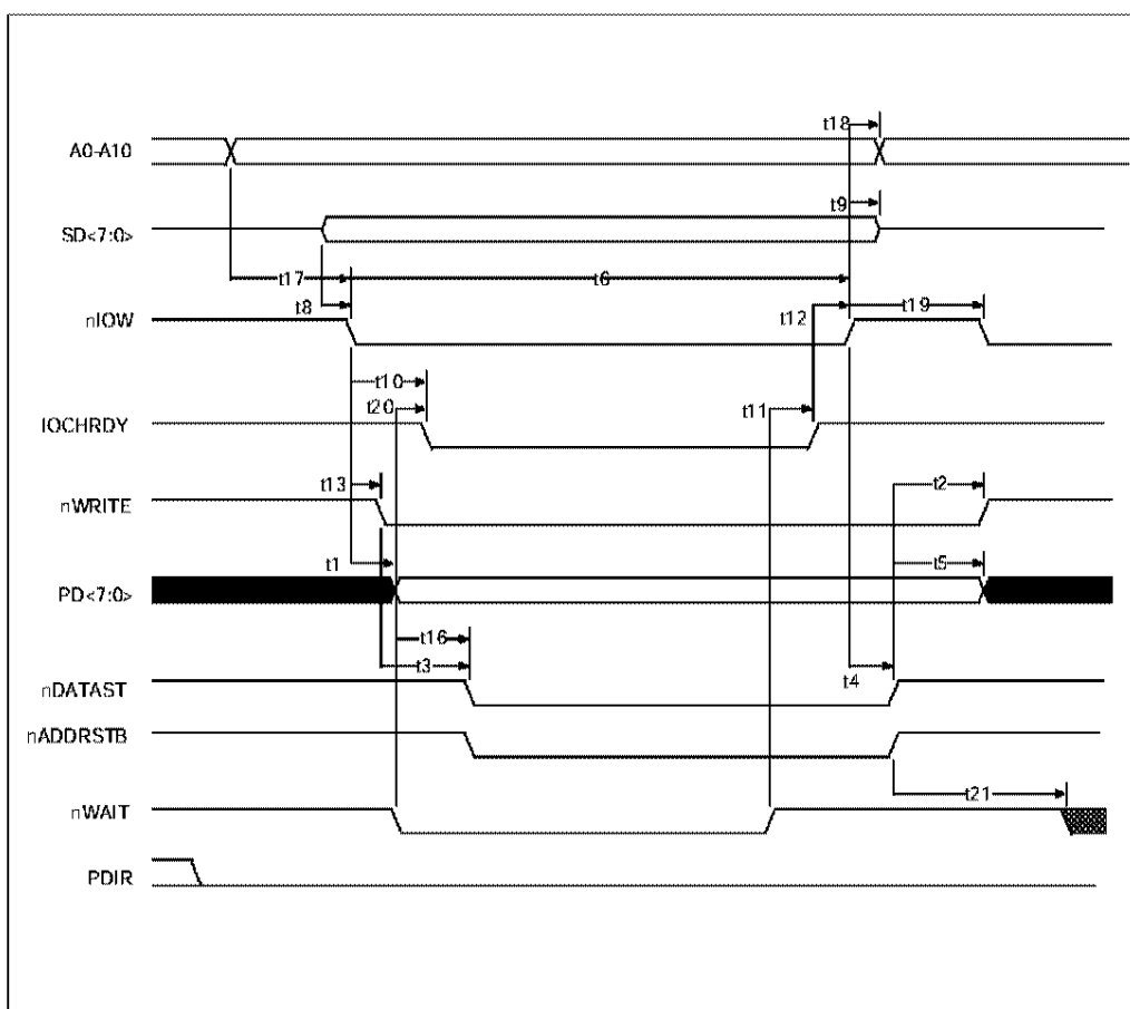
FIGURE 12 - EPP 1.7 DATA OR ADDRESS WRITE CYCLE
