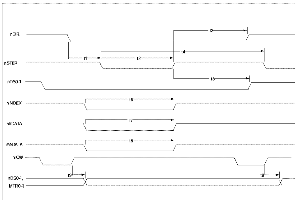
FIGURE 7 - DISK DRIVE TIMING (AT MODE ONLY)
