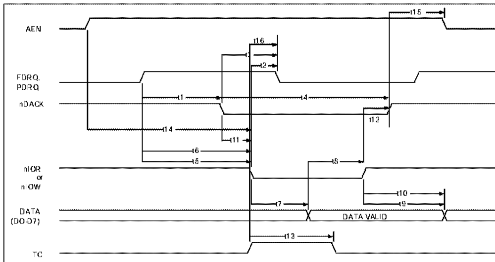
FIGURE 6A - DMA TIMING (SINGLE TRANSFER MODE)
