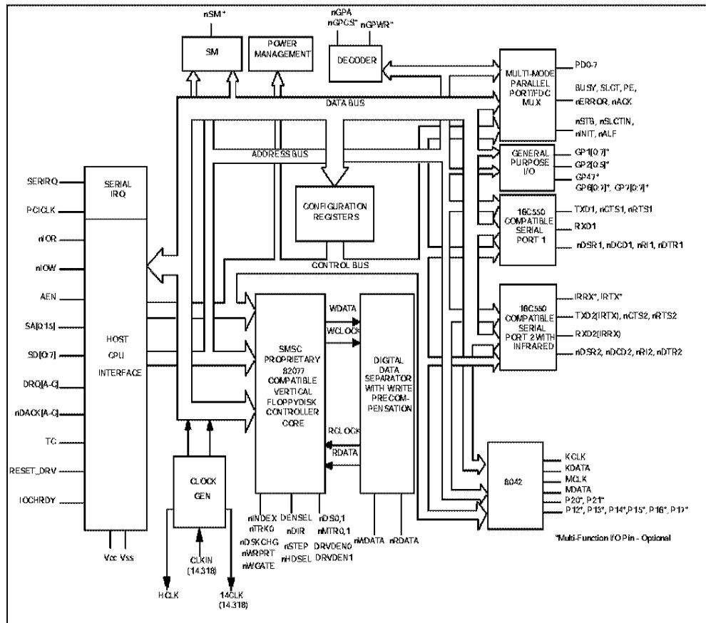
FDC37C68x BLOCK DIAGRAM
