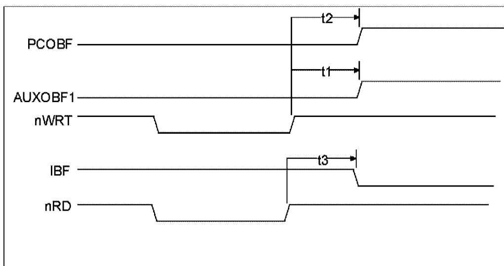
FIGURE 4 - INTERNAL 8042 CPU TIMING
