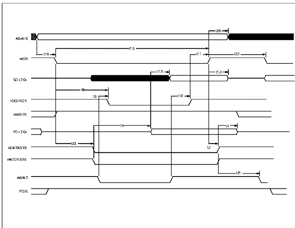
FIGURE 13 - EPP 1.7 DATA OR ADDRESS READ CYCLE
