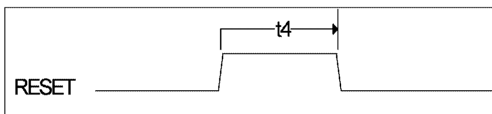
FIGURE 5B - RESET TIMING
