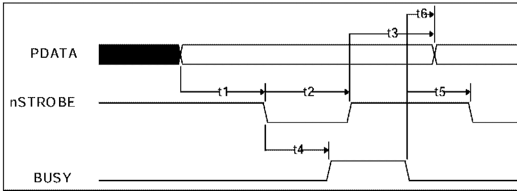
FIGURE 14 - PARALLEL PORT FIFO TIMING
