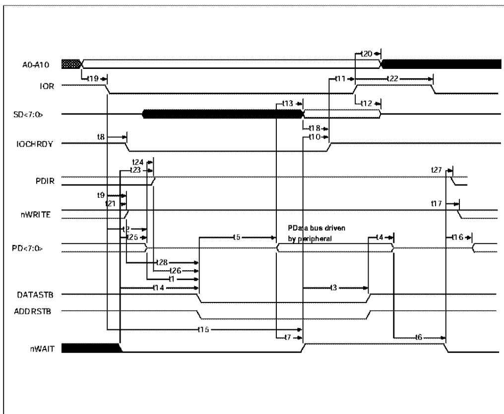
FIGURE 11 - EPP 1.9 DATA OR ADDRESS READ CYCLE
