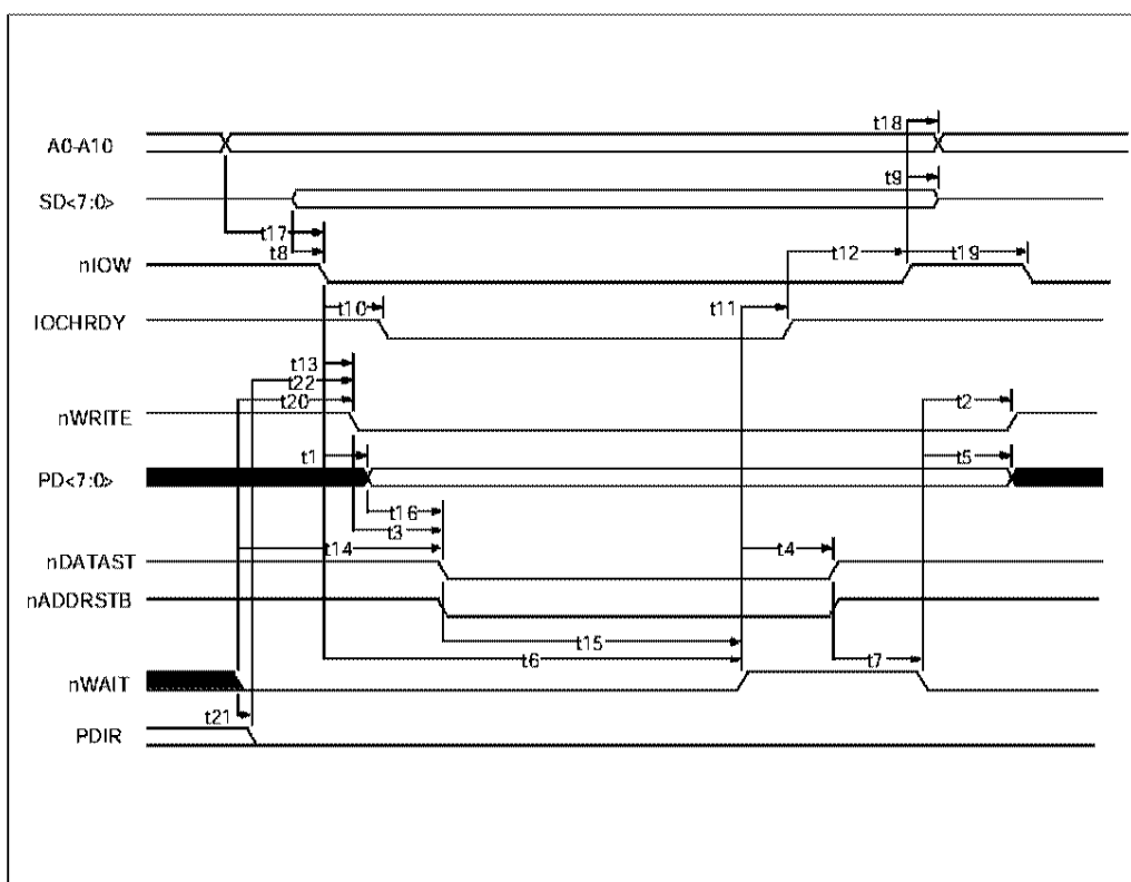
FIGURE 10 - EPP 1.9 DATA OR ADDRESS WRITE CYCLE
