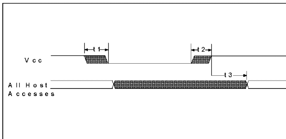
FIGURE 1 - POWER-UP TIMING
