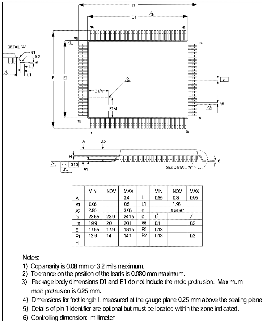
FIGURE 21 - 128 PIN QFP PACKAGE OUTLINES
