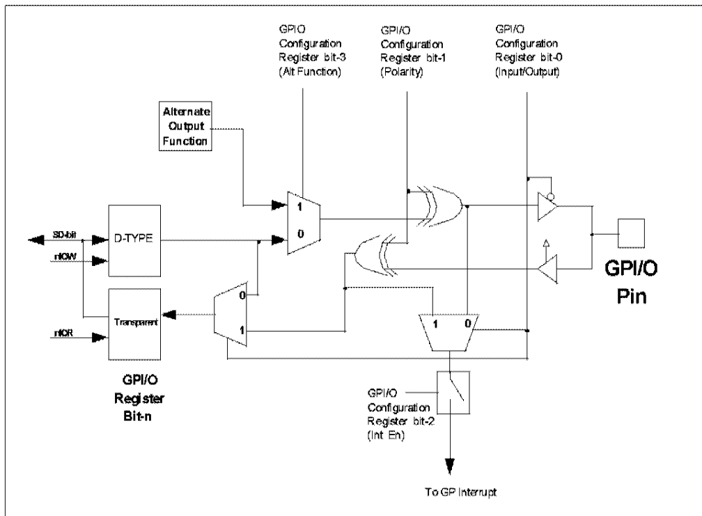
GPIO having an output-type alternate function. [GP12–GP17, GP20, GP22–GP25]
