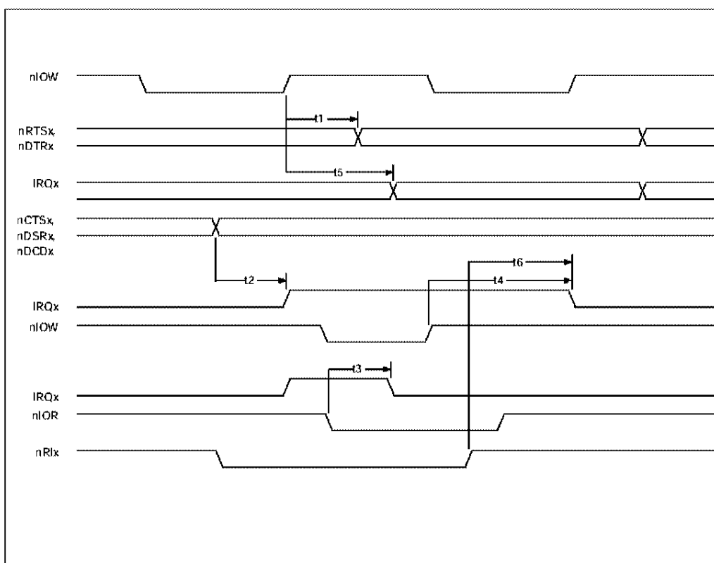
FIGURE 8 - SERIAL PORT TIMING
