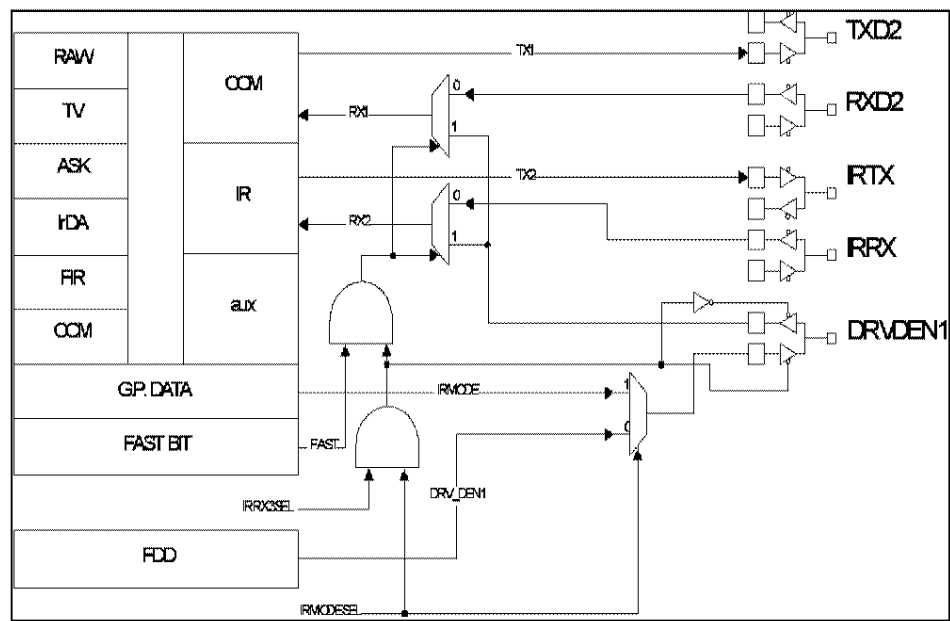
FIGURE 2 - IR INTERFACE BLOCK DIAGRAM
