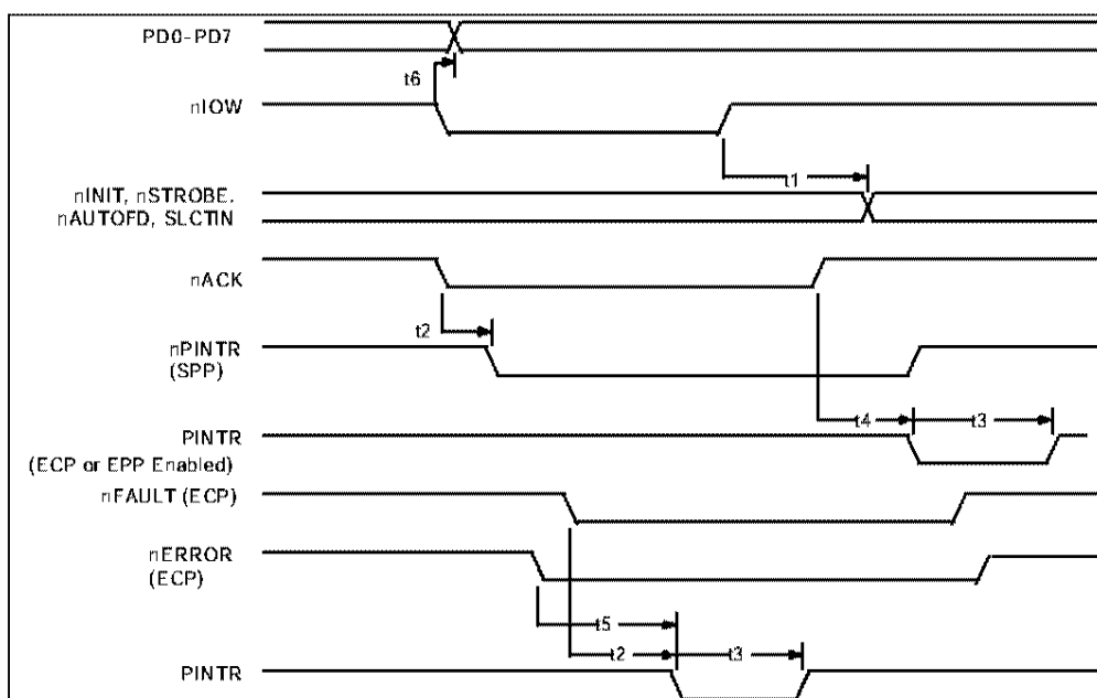
FIGURE 12 - PARALLEL PORT TIMING
