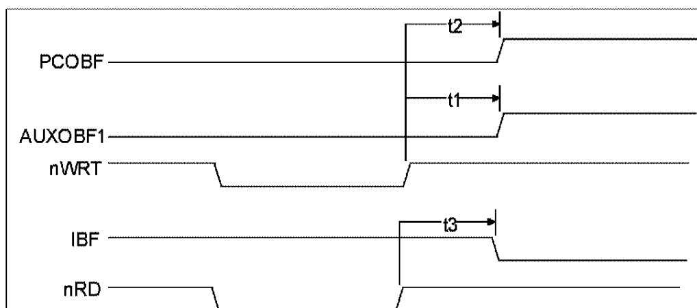
FIGURE 7 - INTERNAL 8042 CPU TIMING
