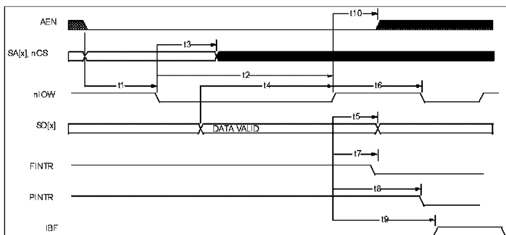
FIGURE 5 - ISA WRITE
