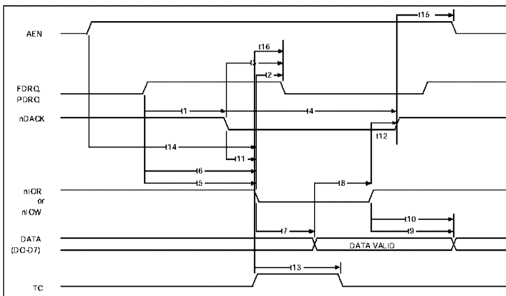
FIGURE 9A - DMA TIMING (SINGLE TRANSFER MODE)
