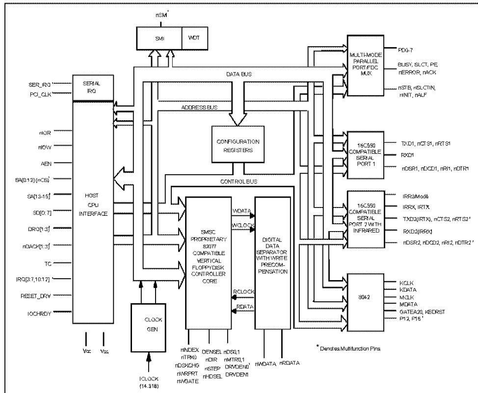
FIGURE 1 - FDC37C67x BLOCK DIAGRAM
