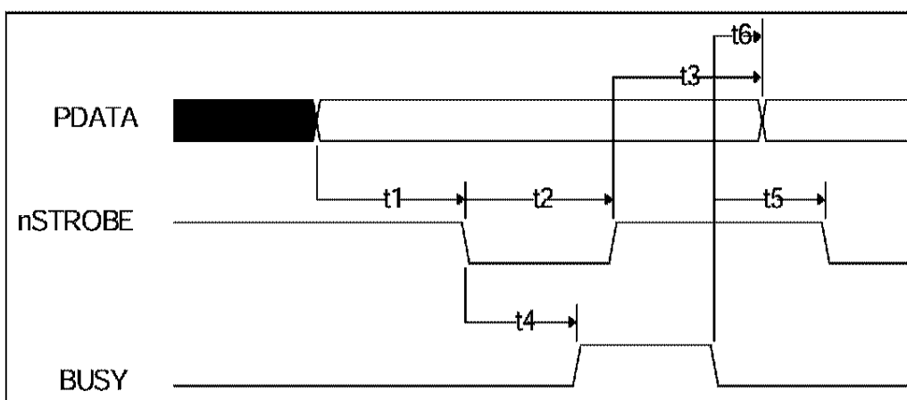
FIGURE 17 - PARALLEL PORT FIFO TIMING
