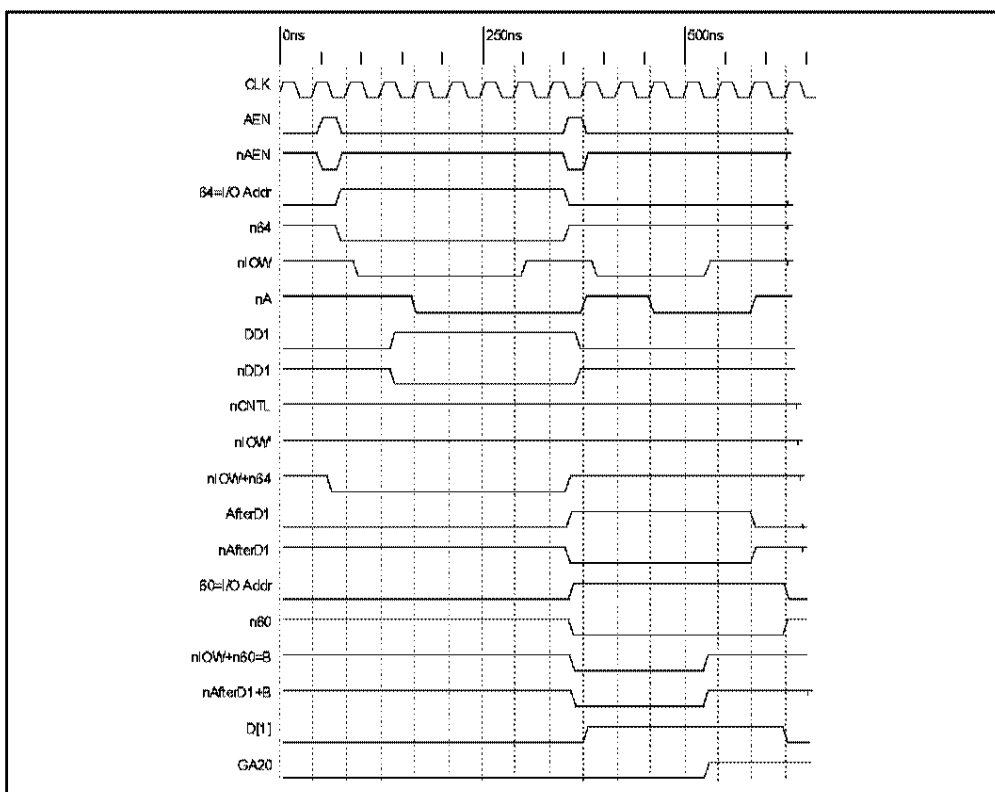
Gate A20 Turn-On Sequence Timing
