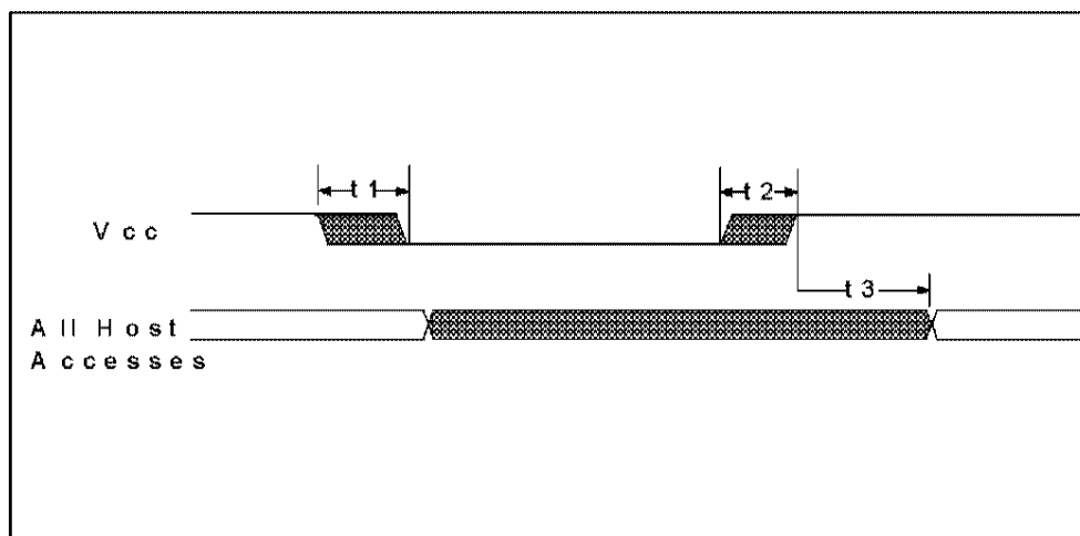
FIGURE 4 - POWER-UP TIMING
