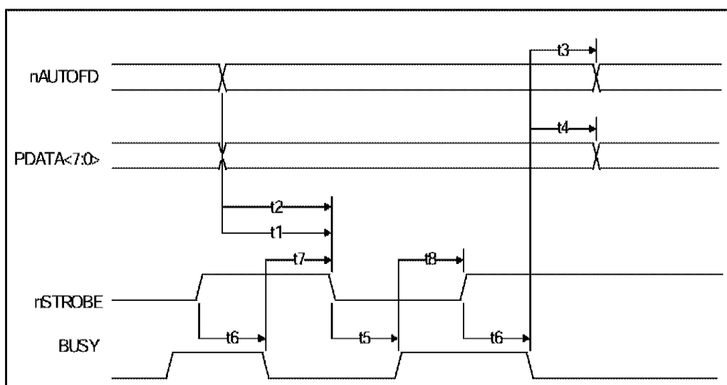
FIGURE 18 - ECP PARALLEL PORT FORWARD TIMING
