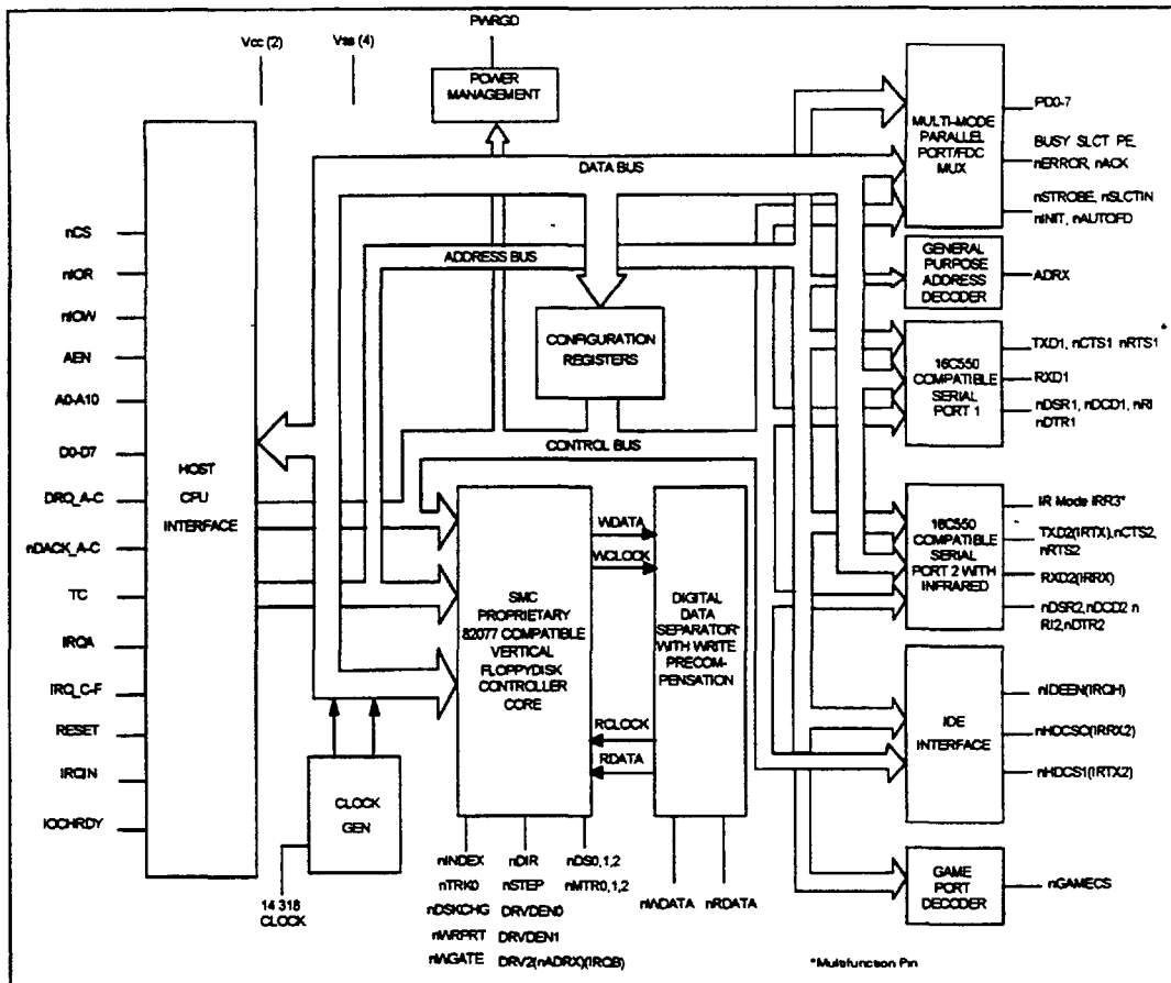
FIGURE 1 - FDC37C669FR BLOCK DIAGRAM
