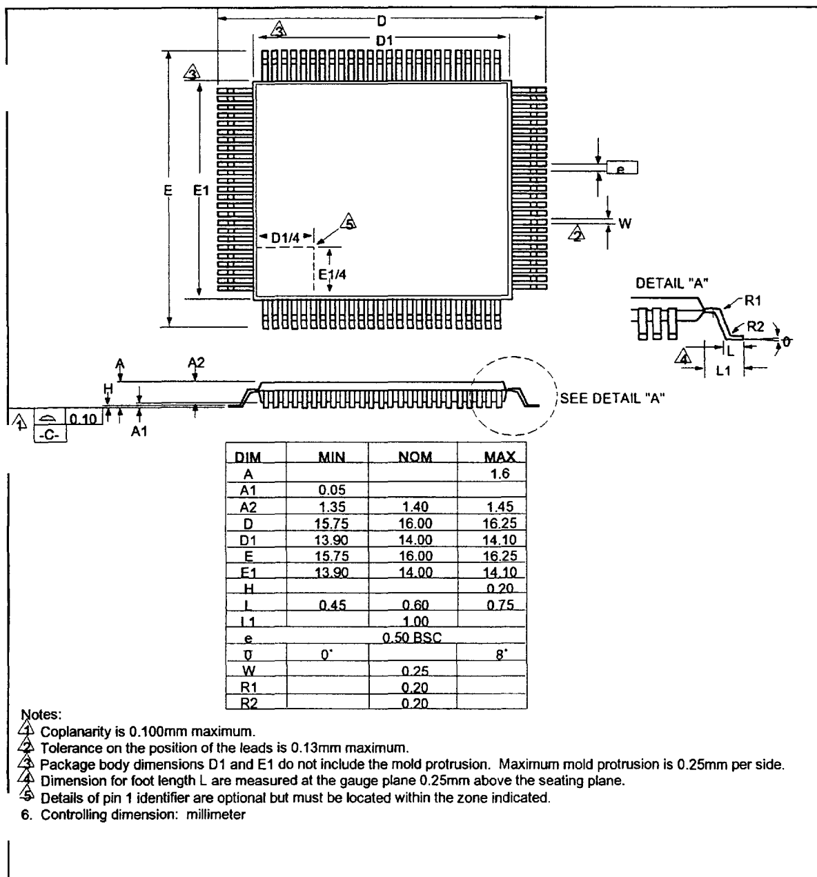
FIGURE 23 - 100 PIN TQFP PACKAGE OUTLINE
